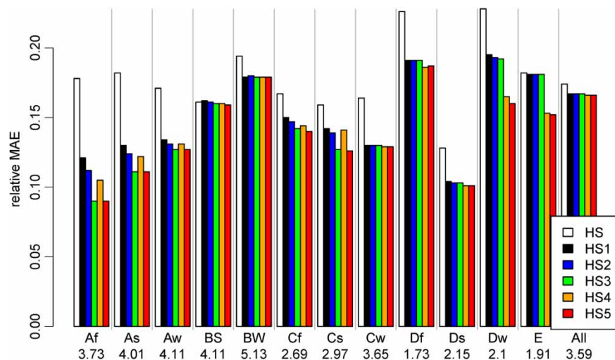
Figure 2 | Relative MAE (MAE over mean ETO per climate class) of HS and various calibrations of HS. Values of mean ETO per climate class in mm day -1 are provided as well.
