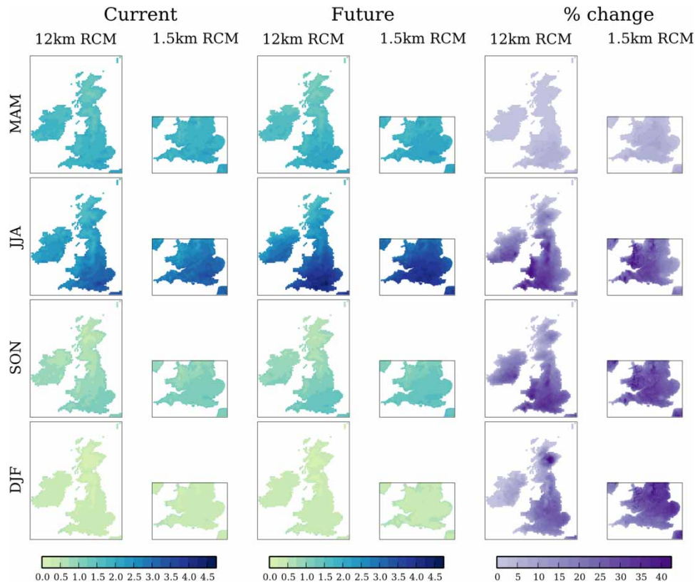
Figure 4 | Seasonal mean PE (mm/day) under climate change, including the effect of changes in stomatal resistance. The averages are for 1997–2008 for the Current RCM and for 12 years in the 2100s for the Future RCM. The percentage change between the Current and Future PE is also shown.
