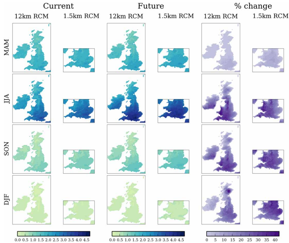
Figure 4 | Seasonal mean PE (mm/day) under climate change, including the effect of changes in stomatal resistance. The averages are for 1997–2008 for the Current RCM and for 12 years in the 2100s for the Future RCM. The percentage change between the Current and Future PE is also shown.
