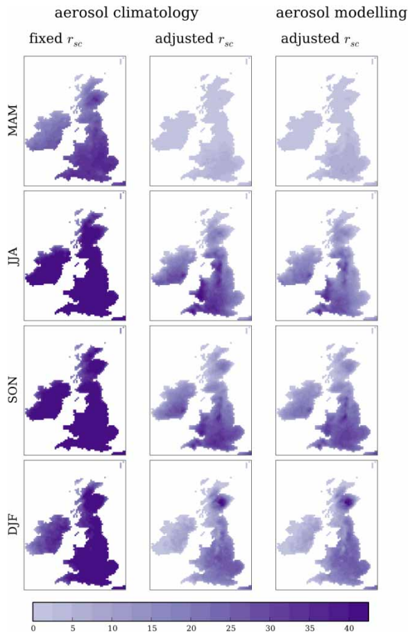
Figure 5 | Seasonal mean percentage change in PE for the 12 km RCM. Left is fixed MORECS r_{sc} for both Current and Future, with aerosol climatology. Middle is MORECS r_{sc} for Current and adjusted r_{sc} for Future, with aerosol climatology. Right is MORECS r_{sc} for Current and adjusted r_{sc} for Future, with full aerosol modelling.
