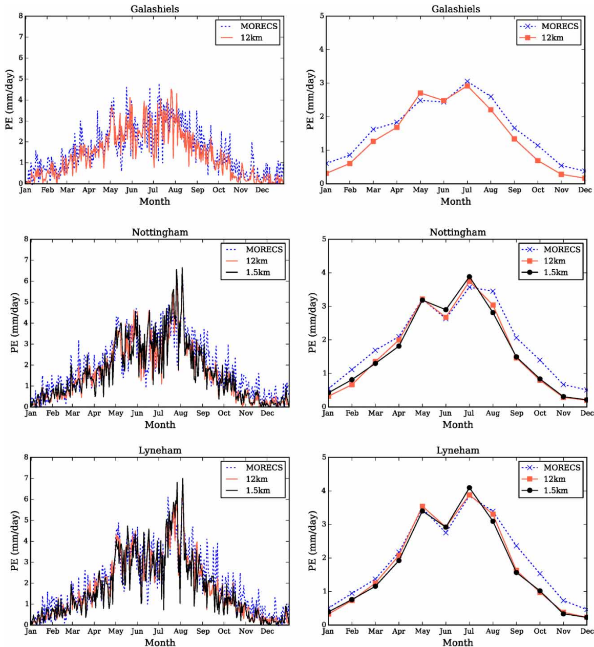
Figure 2 | Comparison of daily and monthly MORECS PE and ERA-driven RCM PE for 1990, for three MORECS sites.
