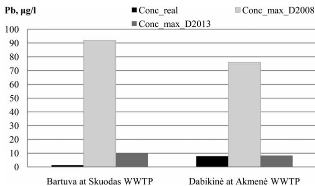
Figure 8 | Real measured (Conc-real), estimated maximum concentrations according to Directive 2008/105/EC (Conc_max_D2008) and Directive 2013/39/EU (Conc_max_D2013) of lead using the mixing zone approach.
