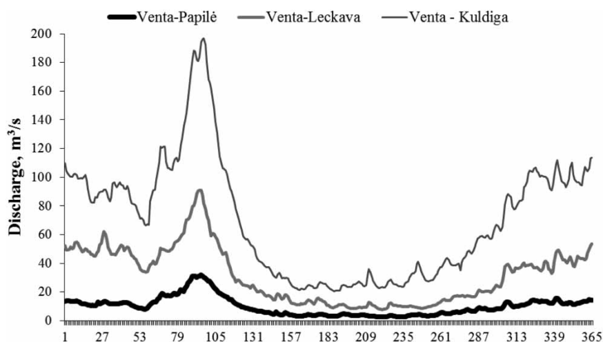
Figure 4 | Runoff distribution (hydrographs) in different gauging stations of the Venta RBD.
