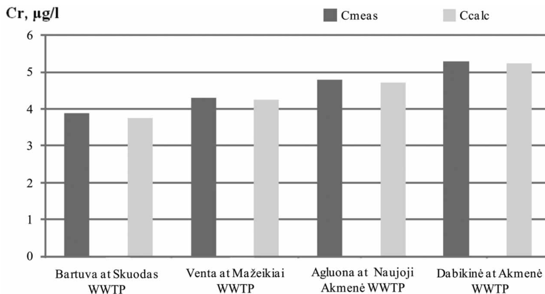
Figure 5 | The measured ( C_{meas} ) and calculated ( C_{calc} ) values of chrome concentrations ( \mu\text{g/L} ) at the end of the predefined mixing zones in four hot spots on the Lithuanian side.
