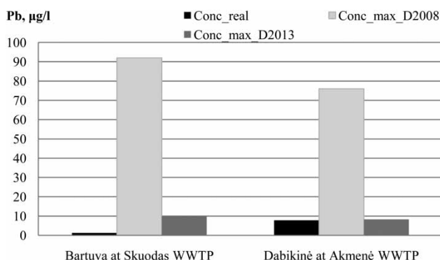
Figure 8 | Real measured (Conc-real), estimated maximum concentrations according to Directive 2008/105/EC (Conc_max_D2008) and Directive 2013/39/EU (Conc_max_D2013) of lead using the mixing zone approach.
