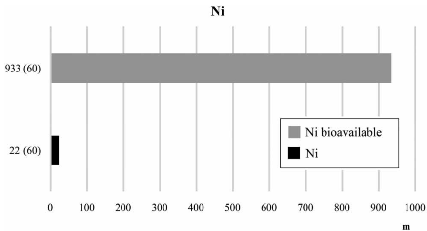
Figure 7 | The lengths of calculated mixing zones for dissolved and bioavailable nickel at 'Aizputes komunālais uzņēmums' in the Tebra: Ni, applied EQS from the 2008/105/EC; Ni bioavailable, applied EQS from the 2013/39/EU.
