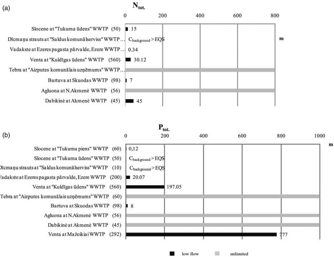
Figure 6 | Comparison of the lengths of calculated mixing zones for nutrients: (a) total nitrogen ( N_{tot} ) and (b) total phosphorus ( P_{tot} ) (in brackets – length of the default mixing zone (value equal to 10 water body widths), another number – length of the calculated real mixing zone bounded by AA-EQS).
