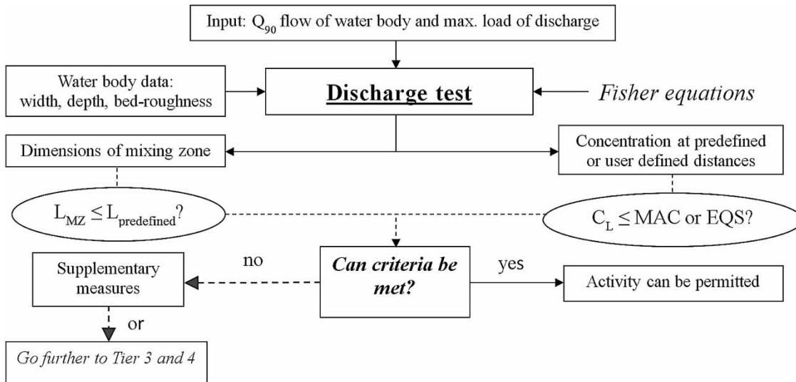
Figure 2 | An overview scheme of the Discharge Test software (according to CIS-WFD (2010) and Ministry of Infrastructure and the Environment (2011)). Max. load of discharge refers to the maximum flow of discharge and effluent concentration.
