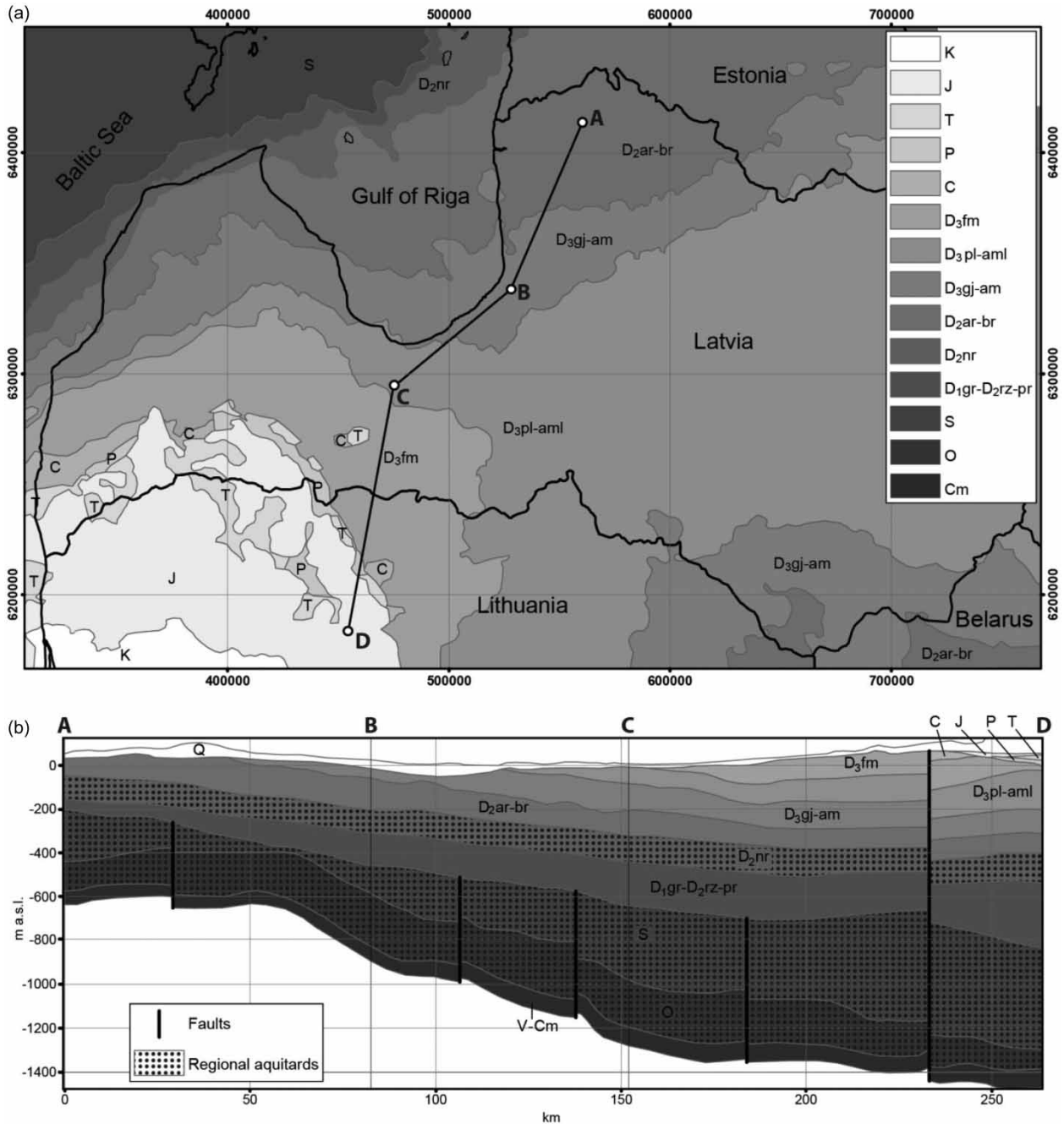
Figure 1 | Geological map and geological cross-section of the study region without Quaternary cover (modified after Virbulis et al. 2013 ; Popovs et al. 2015 ). (a) Geological map. Labelled line denotes location of cross-section. V-Cm, Ediacaran-Cambrian sequence; O, Ordovician sequence; S, Silurian sequence; D 1gr -D 2rz -pr, lower Devonian Gargzdu Fm to middle Devonian Parnu Fm; D 2nr , middle Devonian Narva formation; D 2ar -br, middle Devonian Burnieki Fm to Arukila Fm; D 3gj -am, upper Devonian Gauja Fm to Amata Fm; D 3fm , upper Devonian Famena Fm; C, Carboniferous sequence; P, Permian sequence; T, Triassic sequence; J, Jurassic sequence; K, Cretaceous sequence. (b) Geological cross-section. Thick vertical lines denote major fault structures.
