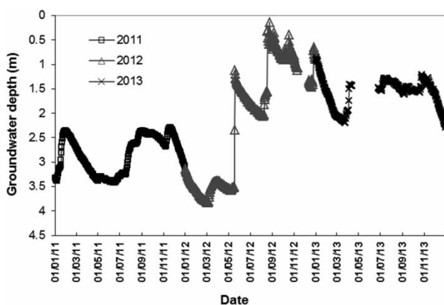
Figure 5 | Groundwater depth registered in borehole No. 31 between 2011 and 2013.
