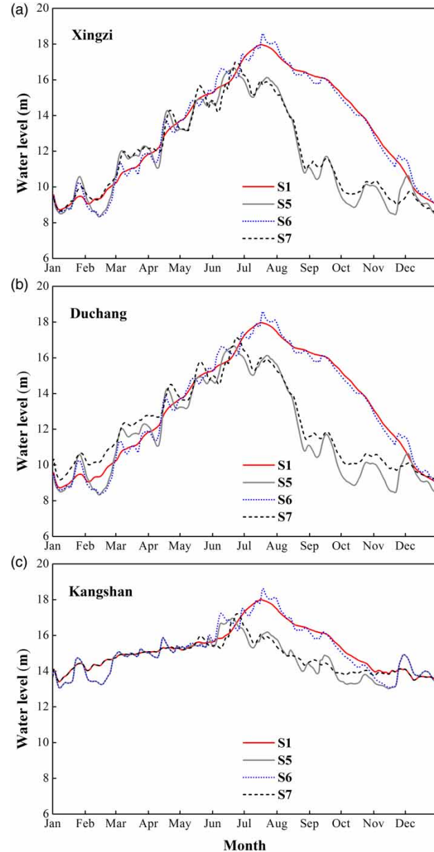
Figure 6 | Comparison of water levels in Scenarios S1, S5, S6, and S7 for (a) Xingzi, (b) Duchang, and (c) Kangshan.
