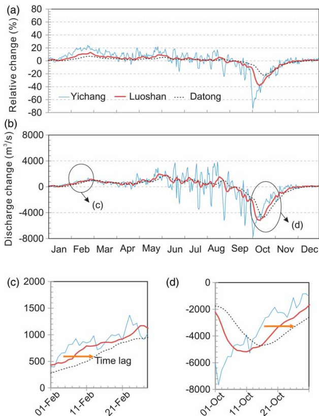
Figure 3 Daily flow alteration in the main stream of the Middle Yangtze induced by the TGD during the years of 2006–2011: (a) relative discharge change at the Yichang, Luoshan, and Datong stations; (b) the absolute discharge change at three stations; (c) zoomed discharge changes show the time-lag of the TGD's impact on the downstream river.
