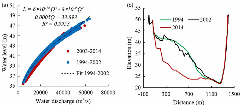
Figure 6 | Water level–discharge rating curves (a) and cross-sectional channel profiles (b) at Zhicheng in 1994–2014.
