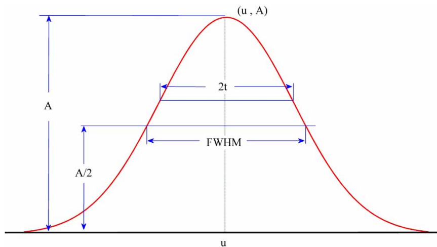
Figure 4 | Sample curve of Gaussian regression.
