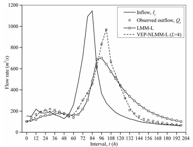
Figure 4 | Observed and estimated outflows for the River Wye, December 1960 flood.
