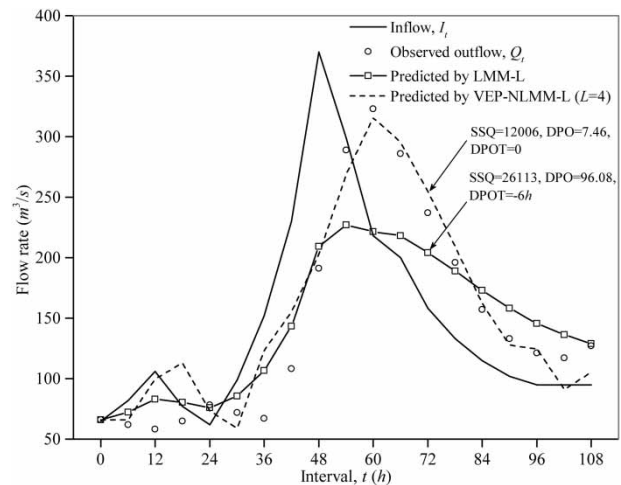
Figure 5 | Observed and predicted outflows for the River Wye, January 1969 flood.
