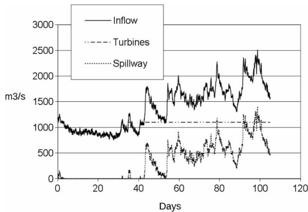
Figure 3 | Time series (05.04.2007–18.07.2007: 105 days) of water discharges in the reservoir and out of the turbines and spillway, respectively.
