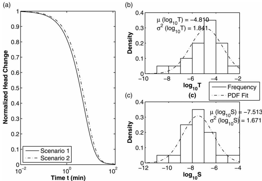
Figure 5 | Fracture model for slug test scenarios: (a) head responses, (b) generated T distribution, and (c) generated S distribution.
