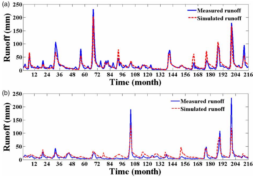
Figure 7 | Hydrographs of observed and simulated monthly runoff during the calibration (a) and validation period (b).
