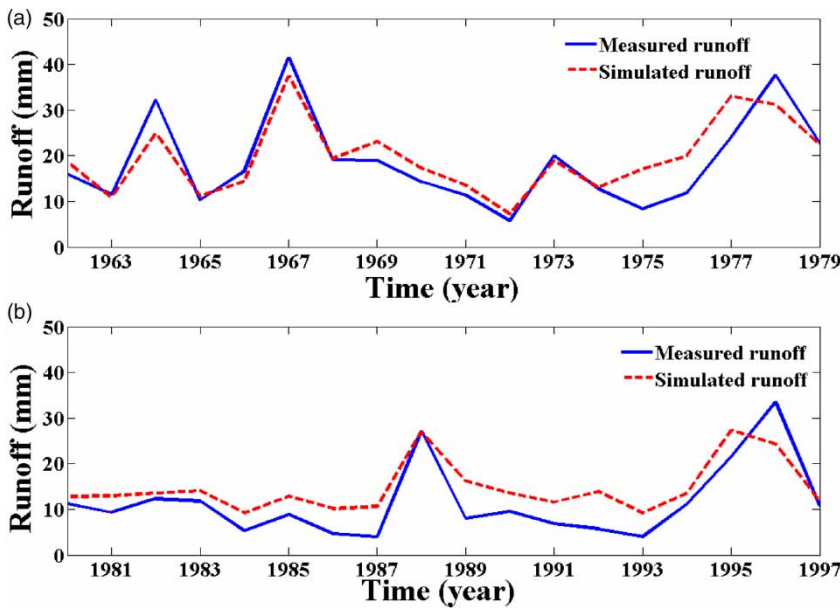
Figure 8 | Hydrographs of observed and simulated annual runoff during calibration (a) and validation period (b).
