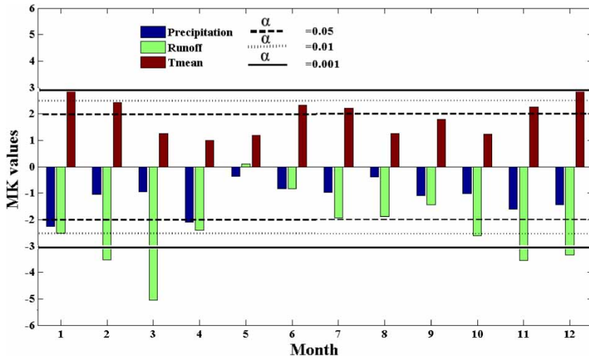
Figure 6 | Mann-Kendall statistics for monthly precipitation, mean temperature, and runoff in HRB during 1961-2000.
