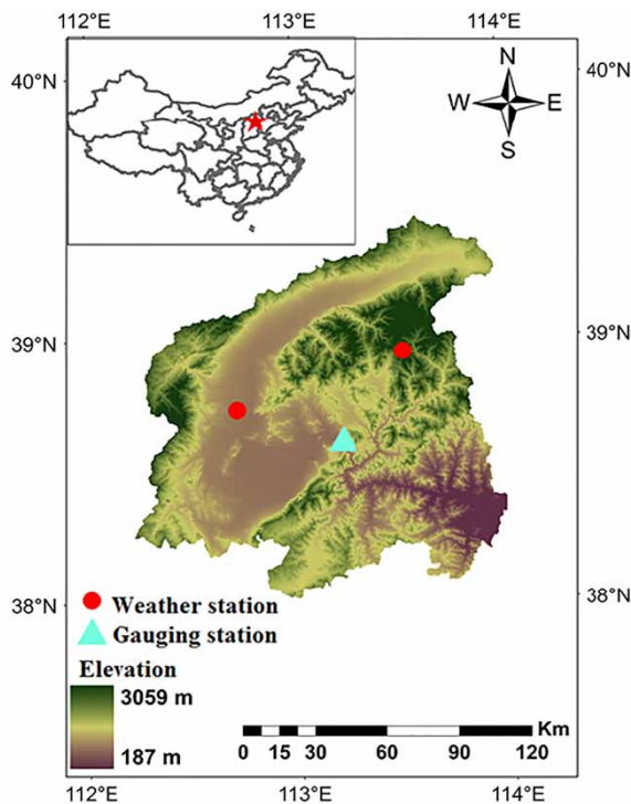
Figure 1 | Location of the study area, gauging station, and weather stations.
