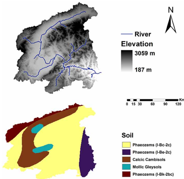
Figure 2 | DEM and soil types in HRB.
