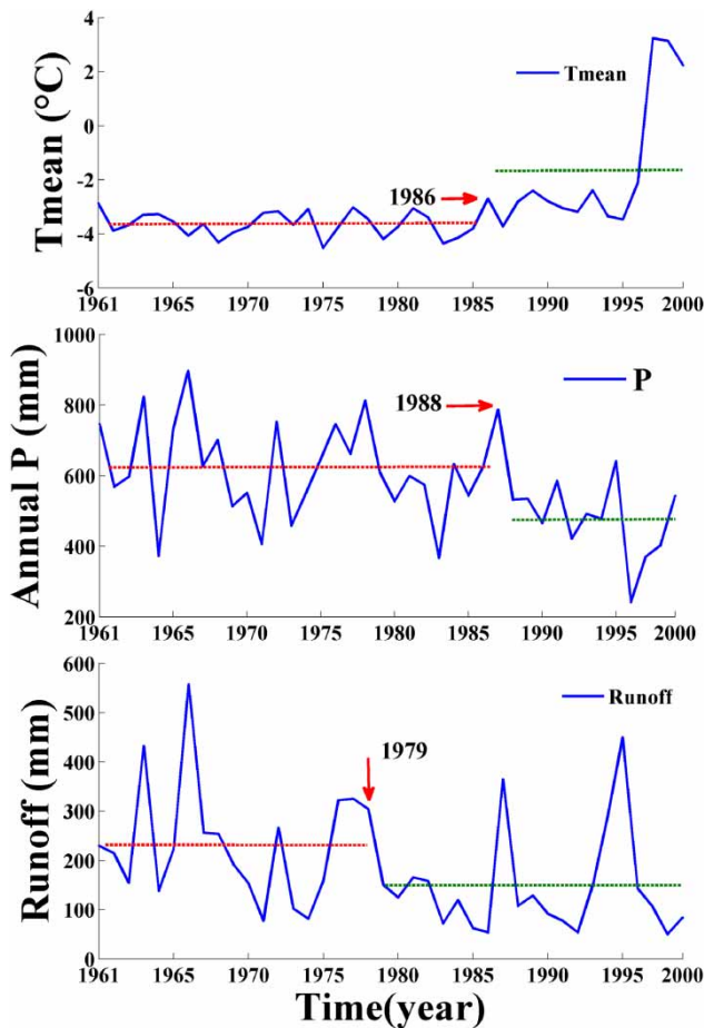
Figure 5 | Change points of annual mean temperature (Tmean), precipitation (P) and runoff time series in HRB during 1961–2000.
