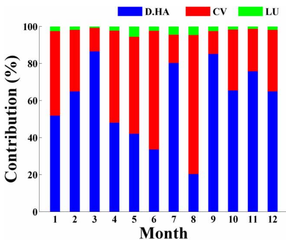
Figure 9 | Contributions of direct human activities (D.H.A), climate variability (CV), and land use (LU) change to average monthly runoff reduction in HRB.
