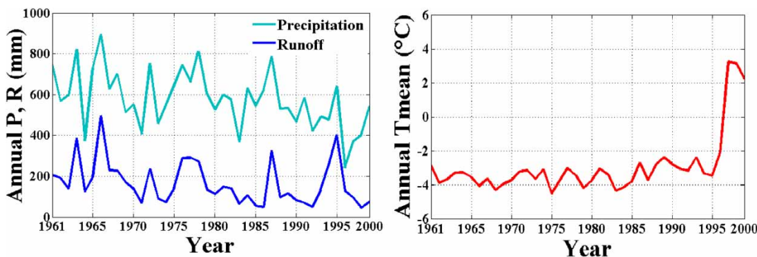
Figure 4 | Time series of annual precipitation (P), runoff (R) and mean temperature (Tmean), from 1961 to 2000 in HRB.
