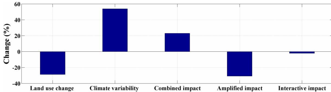
Figure 10 | Evapotranspiration responses to individual and combined impacts of land use and climate variability as well as the amplified impact of land use and the interactive effect of the two factors.
