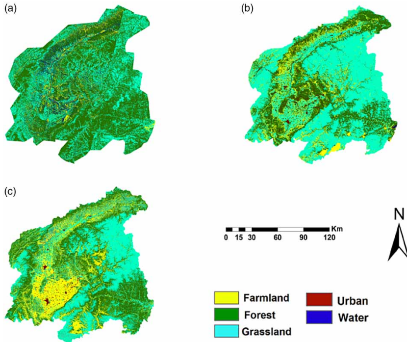
Figure 3 | Land use maps for 1974 (a), 1984 (b), and 2000 (c) in HRB.
