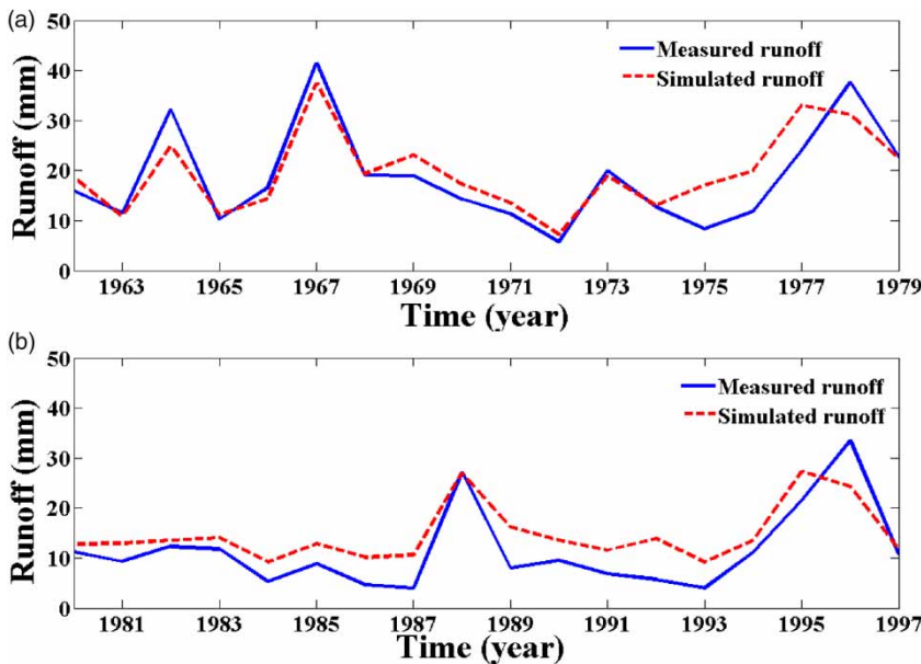
Figure 8 | Hydrographs of observed and simulated annual runoff during calibration (a) and validation period (b).
