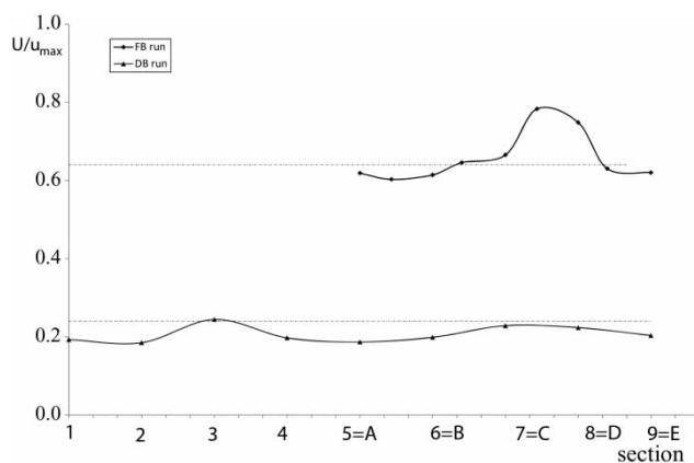
Figure 6 | Ratios U/u_{max} .
