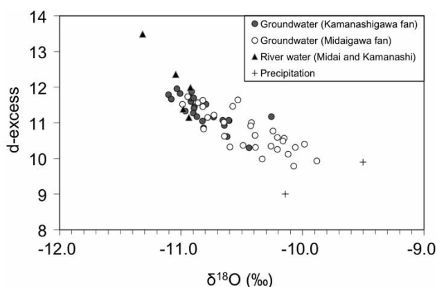
Figure 7 | Plot of d -excess and \delta^{18}\text{O} values of the groundwater, river water, and precipitation samples.
