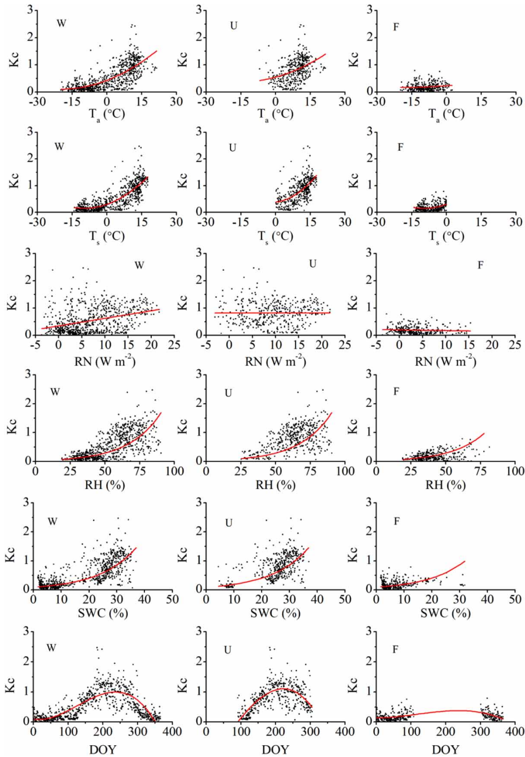
Figure 6 | Regression fitting lines between crop coefficients ( K_c ) and meteorological variables: air temperature ( T_a ), soil surface temperature ( T_s ), RN , RH , soil surface water content ( SWC ), and DOY in different measured periods (W: whole measurement period; U: unfrozen period; F: frozen period).
