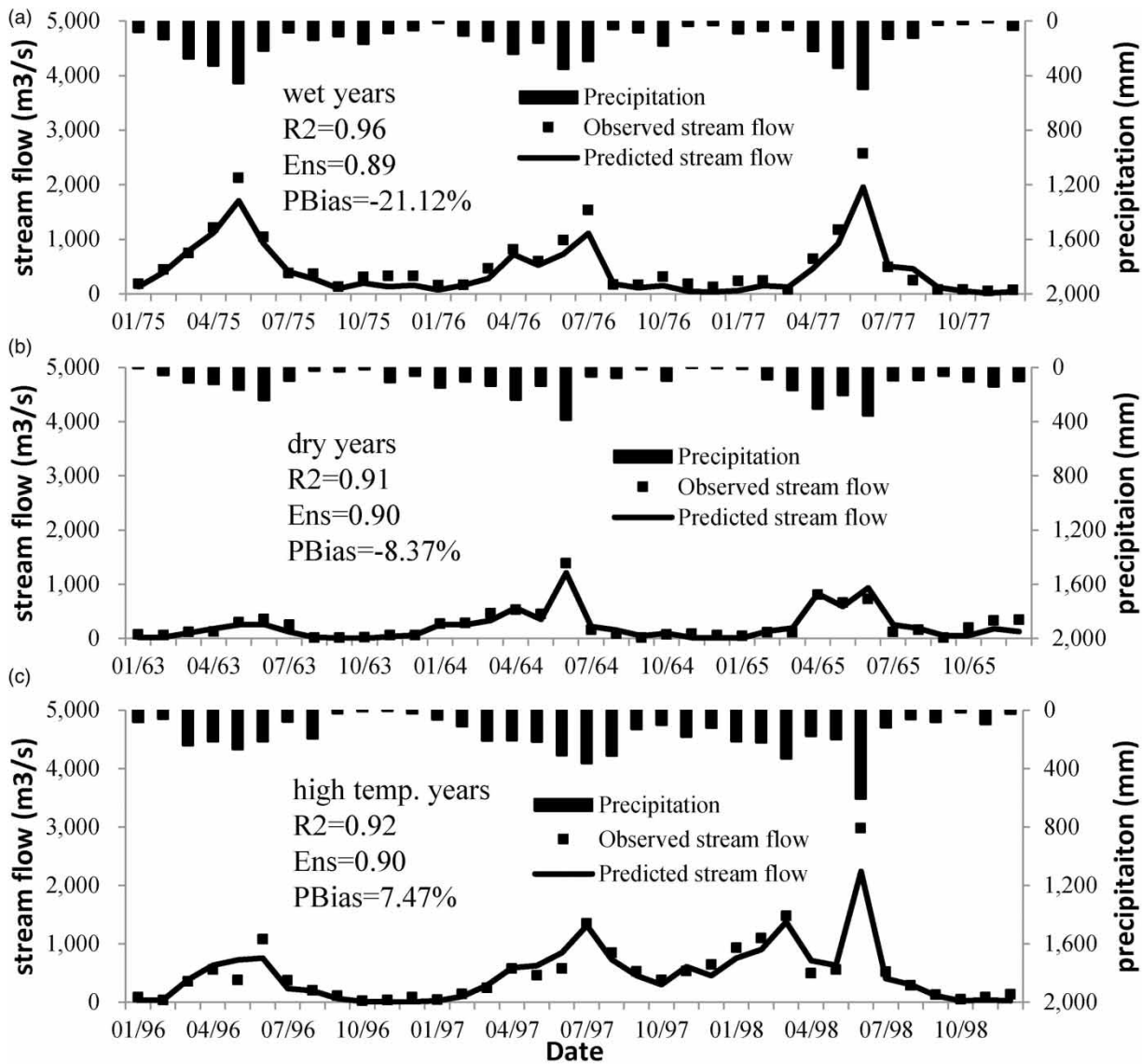
Figure 6 | Validation of stream flow from SWAT model calibrated in the average years: (a) validation in wet years; (b) validation in dry years; (c) validation in high temperature years.
