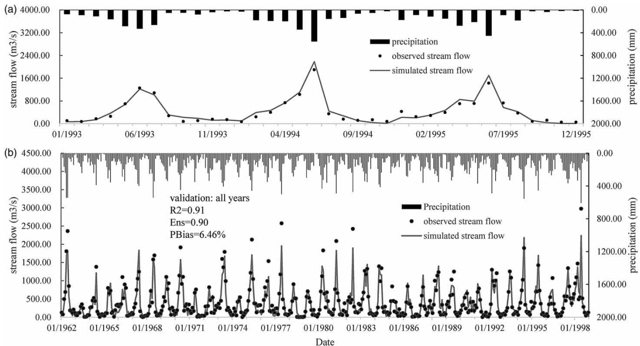
Figure 5 | Comparison between monthly simulated and observed stream flow: (a) calibration in average years; (b) validation for the whole period (1962–1998) under calibrated parameters by data in average years.
