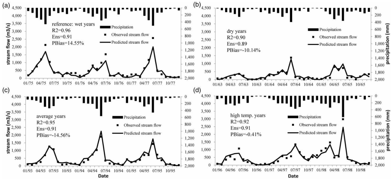
Figure 7 | Hydrological responses to the parameters calibrated in wet years in the Fuhe basin: (a) calibration period; (b) validation in dry years; (c) validation in average years; (d) validation in high temperature years.
