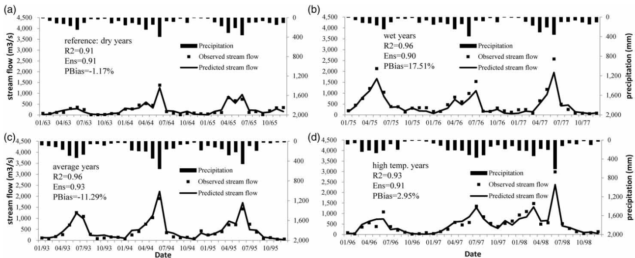
Figure 8 | Hydrological responses to the parameters calibrated in dry years in the Fuhe basin: (a) calibration period; (b) validation in wet years; (c) validation in average years; (d) validation in high temperature years.
