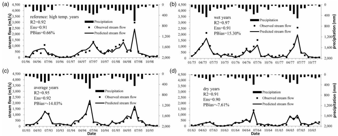
Figure 9 | Hydrological responses to the parameters calibrated in high temperature years in the Fuhe basin: (a) calibration period; (b) validation in wet years; (c) validation in average years; (d) validation in dry years.
