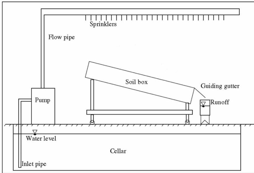
Figure 1 | The simulated rainfall experimental facility.
