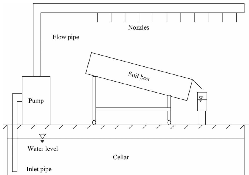
Figure 1 | The schematic diagram of the rainfall simulator.
