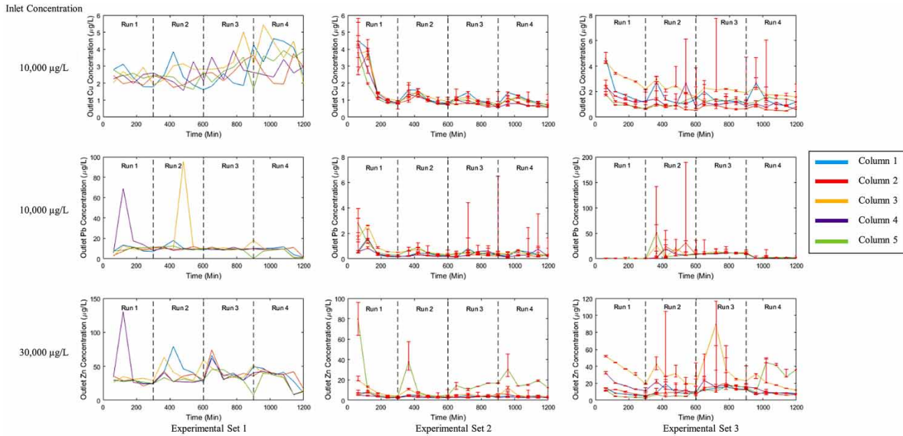
Figure 5 | Heavy metal outflow concentrations for all experiment sets.
