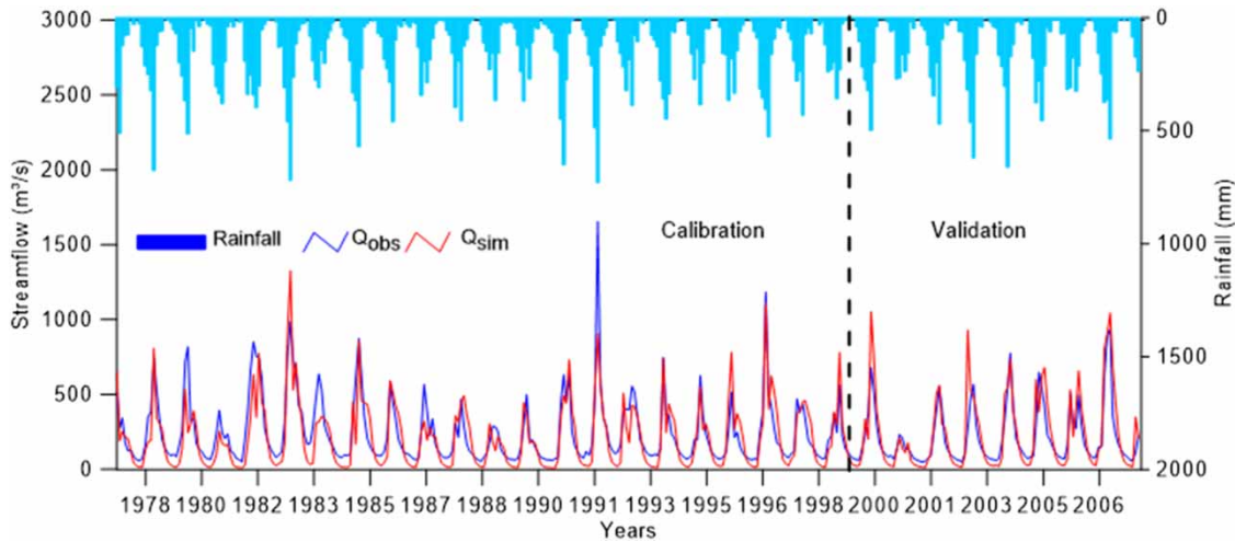
Figure 5 | Simulated and observed monthly runoff and observed hyetograph at the Porto das Andorinhas station.
