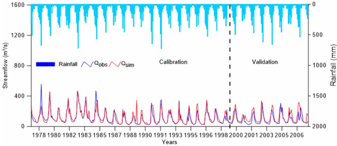
Figure 6 | Simulated and observed monthly runoff and observed hyetograph at the Pari station.
