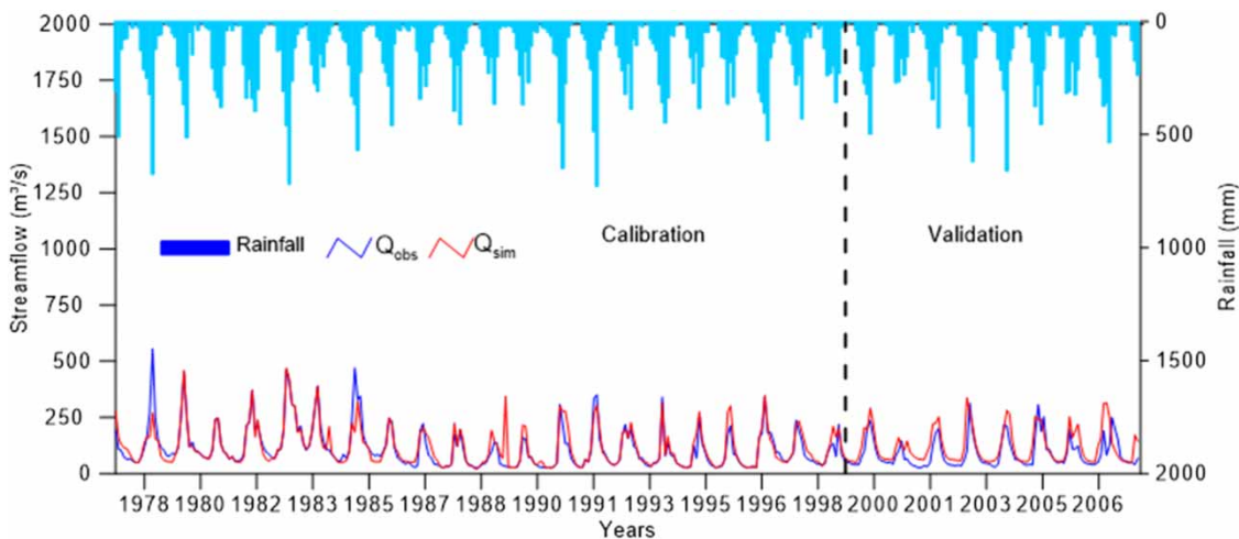
Figure 7 | Simulated and observed monthly streamflow and observed hyetograph at the Ponte da Taquara station.
