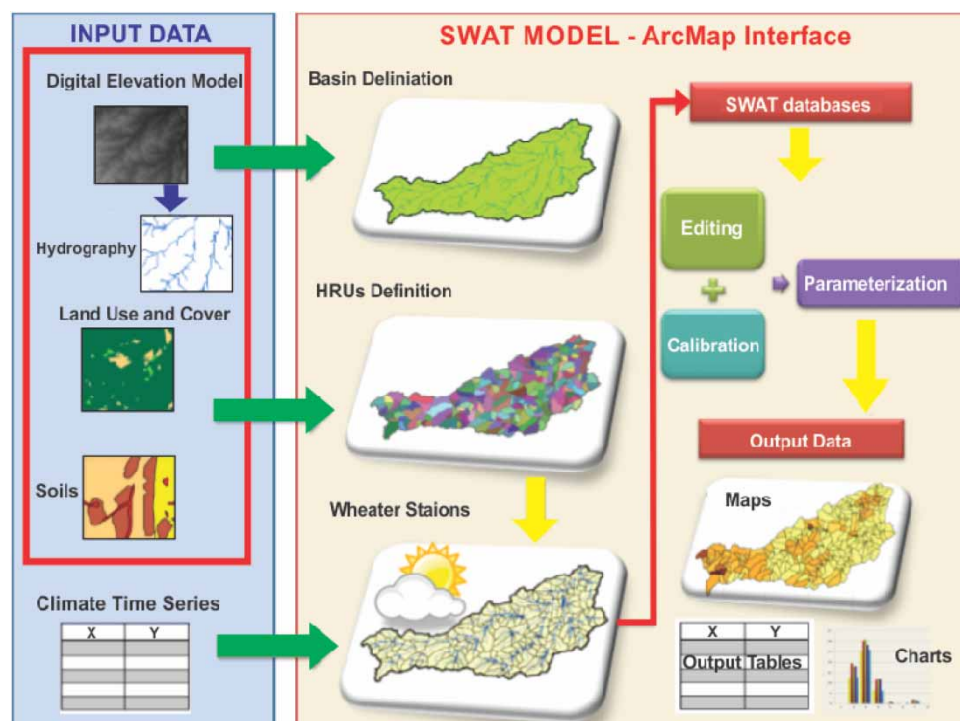
Figure 4 | Schematic framework of the SWAT model.
