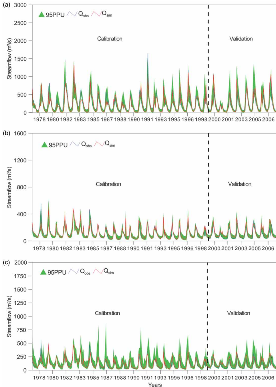
Figure 8 | 95% probability uncertainty plot observed and simulated streamflow for stations: (a) Porto das Andorinhas, (b) Pari and (c) Ponte da Taquara.
