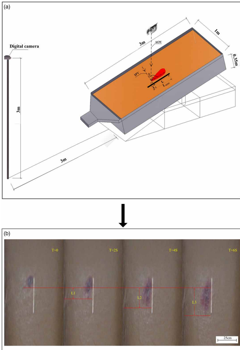
Figure 1 | A schematic for the experiment (a) and the determination of runoff velocity under the integrated dye tracer and image processing method (b).
