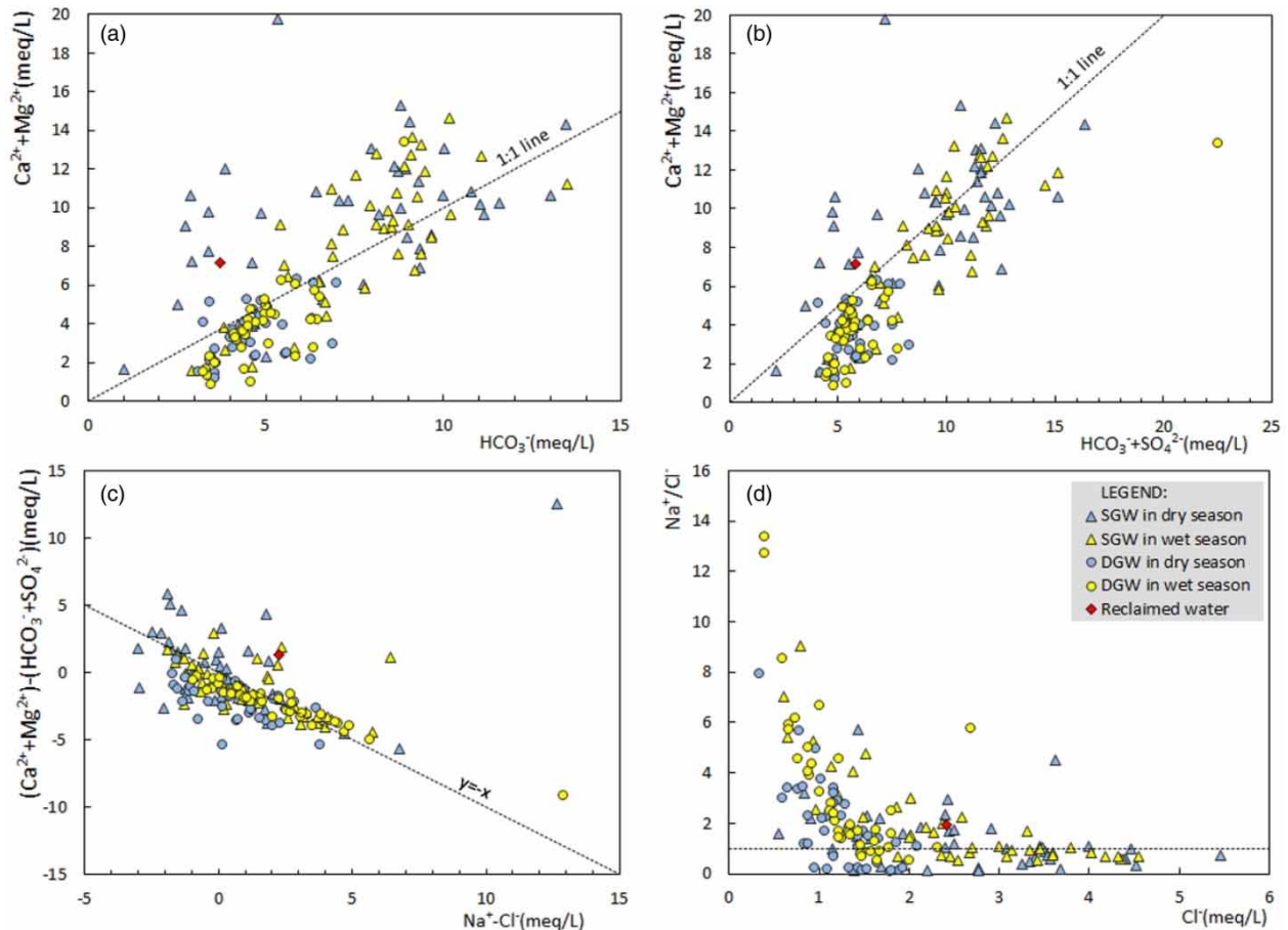
Figure 4 | Plots of ionic ratio between different cations and anions: (a) (Ca^{2+} + Mg^{2+}) versus HCO_3^- ; (b) (Ca^{2+} + Mg^{2+}) versus (HCO_3^- + SO_4^{2-}) ; (c) (Ca^{2+} + Mg^{2+}) - (HCO_3^- + SO_4^{2-}) versus (Na^+ - Cl^-) ; and (d) Na^+/Cl^- versus Cl^- .
