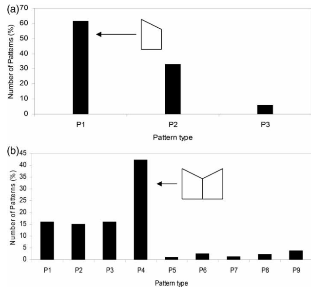
Figure 8 | Percentage of patterns identified in the time series for (a) input structure (number of lags = 1) and (b) input structure (number of lags = 2) for Little River, Virginia, and dominant patterns.
