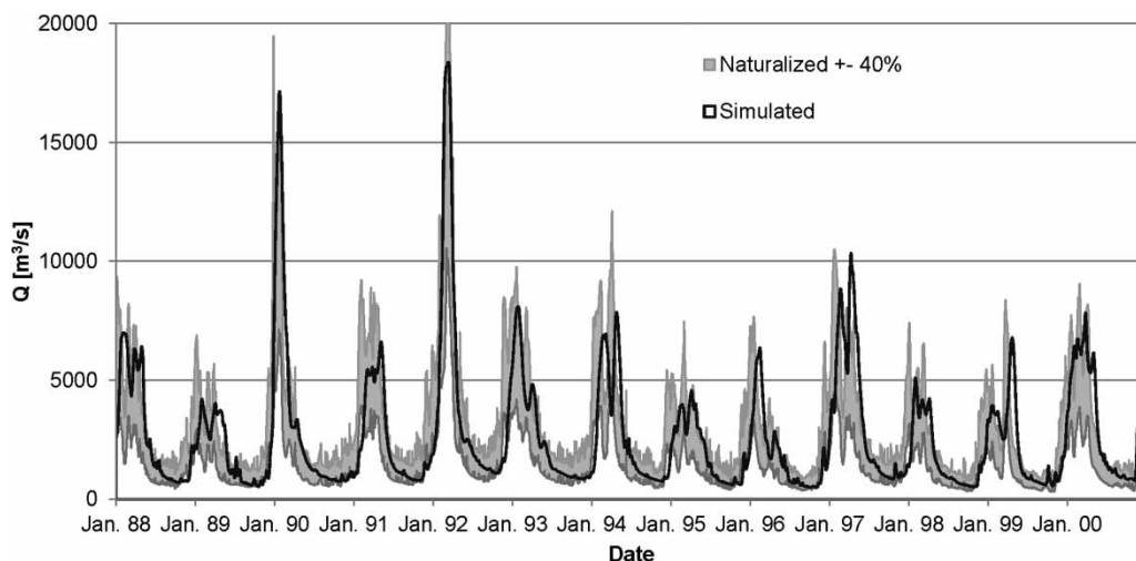
Figure 4 | Naturalized (ONS) and simulated (SWIM) discharges at gauge Xingó (No. 16 in Figure 1).
