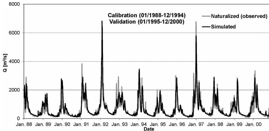
Figure 3 | Naturalized (ONS) and simulated (SWIM) discharges at Trés Marias reservoir.
