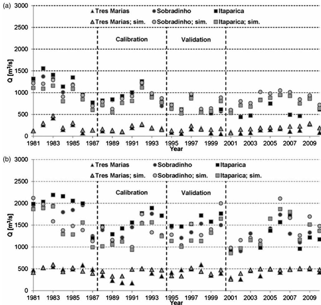
Figure 6 | MAM7-indices for years 1981 to 2010, observed (ONS), and simulated (SWIM) for (a) natural and (b) managed flow.
