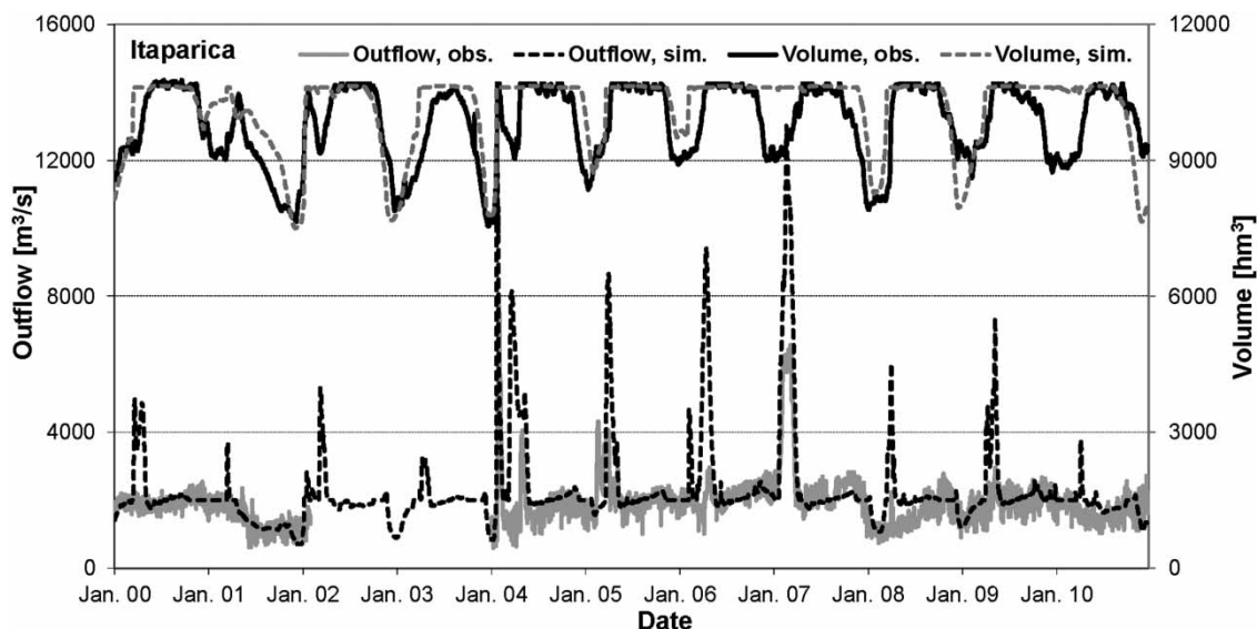
Figure 5 | Observed (ONS) and simulated (SWIM) outflows and volumes for Itaparica reservoir.
