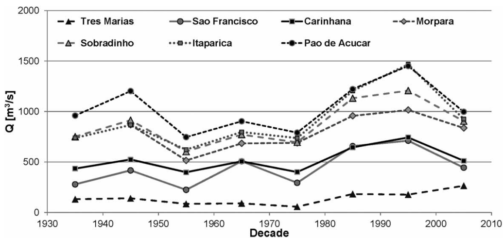
Figure 2 | Development of low flow indices (7Q10) for selected gauges for the decades between 1931 and 2010 (the value placed at year 1935 represents the 7Q10 for the decade 1931–1940, etc.; for location of gauges see Figure 1).
