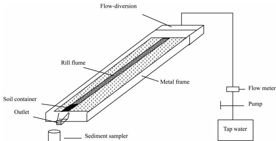
Figure 1 | Experimental devices.
