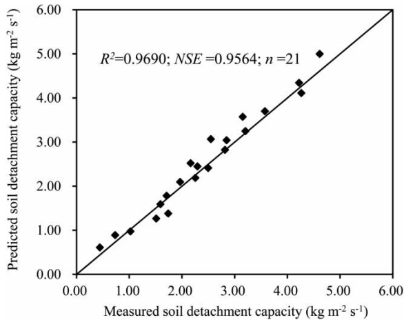
Figure 5 | Measured vs. predicted soil detachment capacity for the validation datasets using the model: D_c = 76.5904S^{1.0148}Q^{1.1224} .
