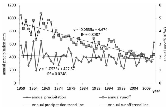
Figure 2 | Temporal change of annual runoff and precipitation during 1959–2012.
