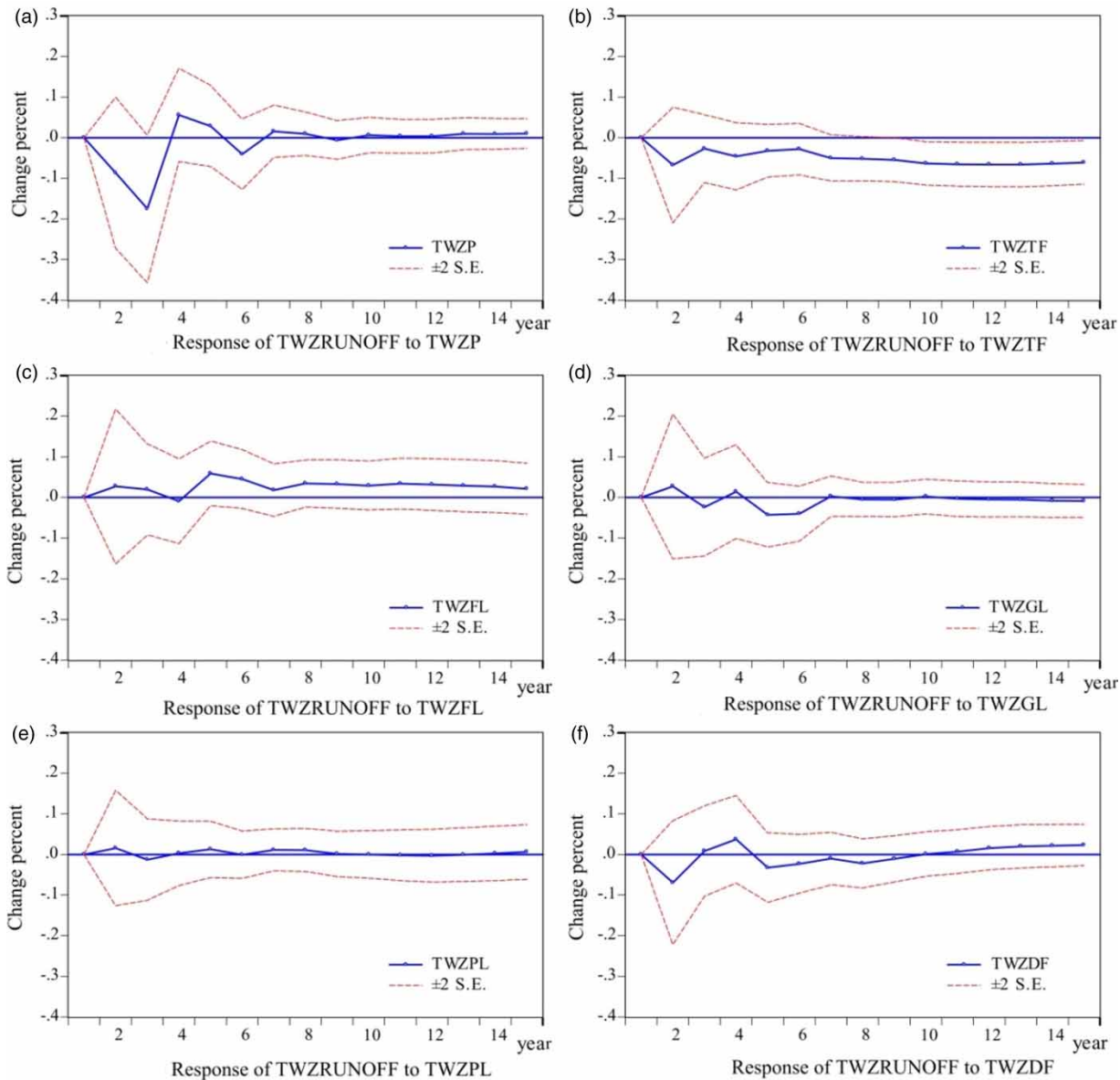
Figure 4 | Response of TWZRUNOFF to relative factors.
