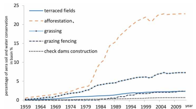
Figure 3 | The percentage of soil and water conservations in the Tuwei River basin during 1959–2012.
