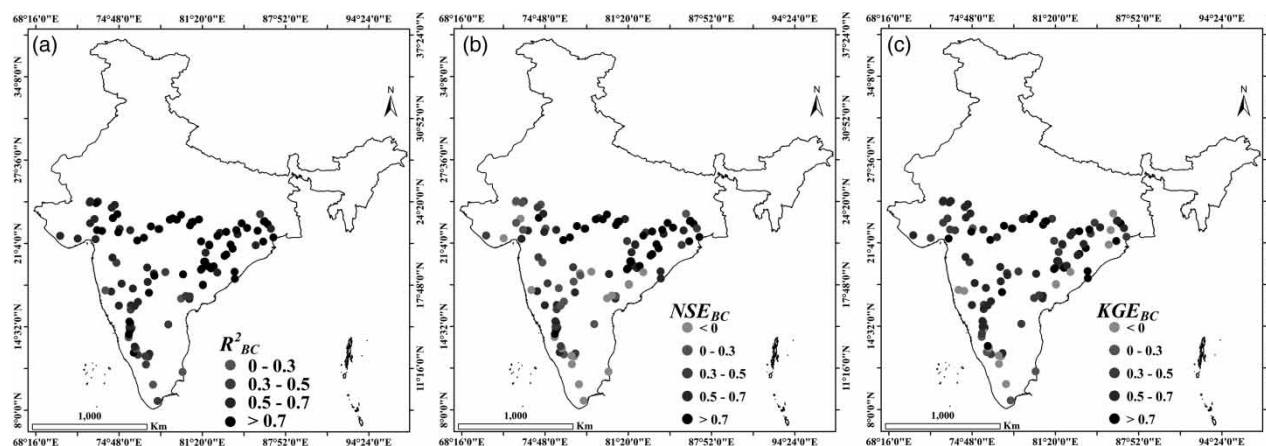
Figure 5 | Maps of the three performance metrics for the study catchments obtained after Box-Cox transformation of discharge: (a) coefficient of determination ( R_{BC}^2 ), (b) Nash-Sutcliffe efficiency ( NSE_{BC} ) and (c) Kling-Gupta efficiency ( KGE_{BC} ).
