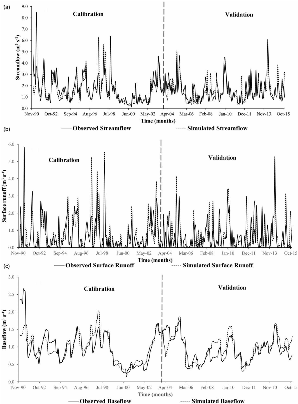
Figure 3 | Observed vs. simulated: (a) streamflow ( \text{m}^3 \text{s}^{-1} ), (b) surface runoff ( \text{m}^3 \text{s}^{-1} ), and (c) baseflow ( \text{m}^3 \text{s}^{-1} ).
