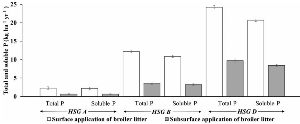
Figure 7 | Average annual (1991–2015) total and soluble P losses ( \text{kg ha}^{-1} \text{yr}^{-1} ) in surface runoff from pastures at the HRU level from soils of different HSGs as a function of surface and subsurface application of broiler litter. Each half bar represents one standard error.
