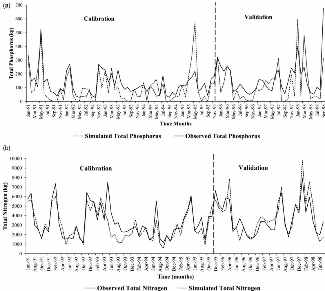
Figure 4 | Observed vs. simulated monthly: (a) P and (b) N loading (kg) at the watershed outlet.
