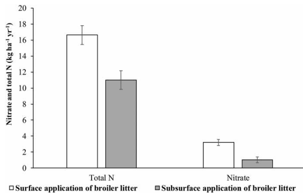
Figure 6 | Average annual (1991–2015) total N and nitrate losses ( \text{kg ha}^{-1} \text{yr}^{-1} ) from pasture HRUs in surface runoff as a function of surface and subsurface application of broiler litter. Each half bar represents one standard error.
