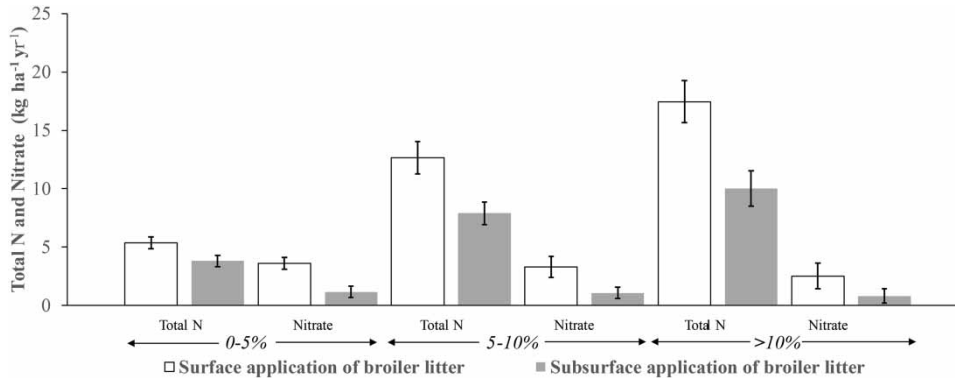
Figure 10 | Average annual (1991–2015) total N and nitrate losses ( \text{kg ha}^{-1} \text{yr}^{-1} ) in surface runoff from pastures at the HRU level from soils on different slope classes as a function of surface and subsurface application of broiler litter. Each half bar represents one standard error.
