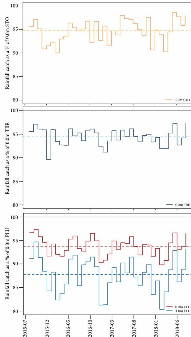
Figure 2 | Monthly undercatch in each raingauge, calculated as a percentage of the rainfall recorded in the reference gauge of that type (mounted at 0.0 m).
