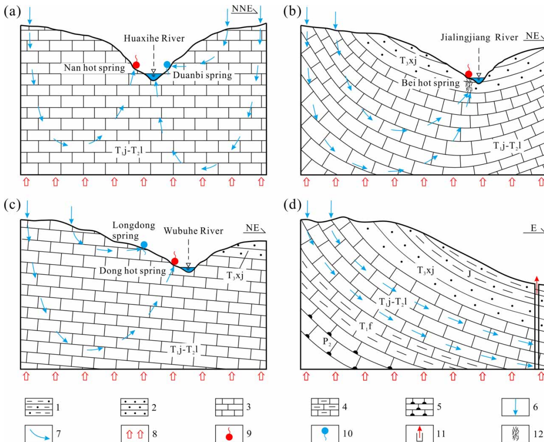
Figure 5 | Schematic profiles showing genesis of the hot springs near Chongqing. 1 Sandy mudstone; 2 Sandstone; 3 Carbonate; 4 Marl; 5 Chert nodule limestone; 6 Infiltration of precipitation; 7 Groundwater flow direction; 8 Heat flow; 9 Natural hot spring; 10 Normal temperature spring; 11 Geothermal well; 12 Fracture zone.
