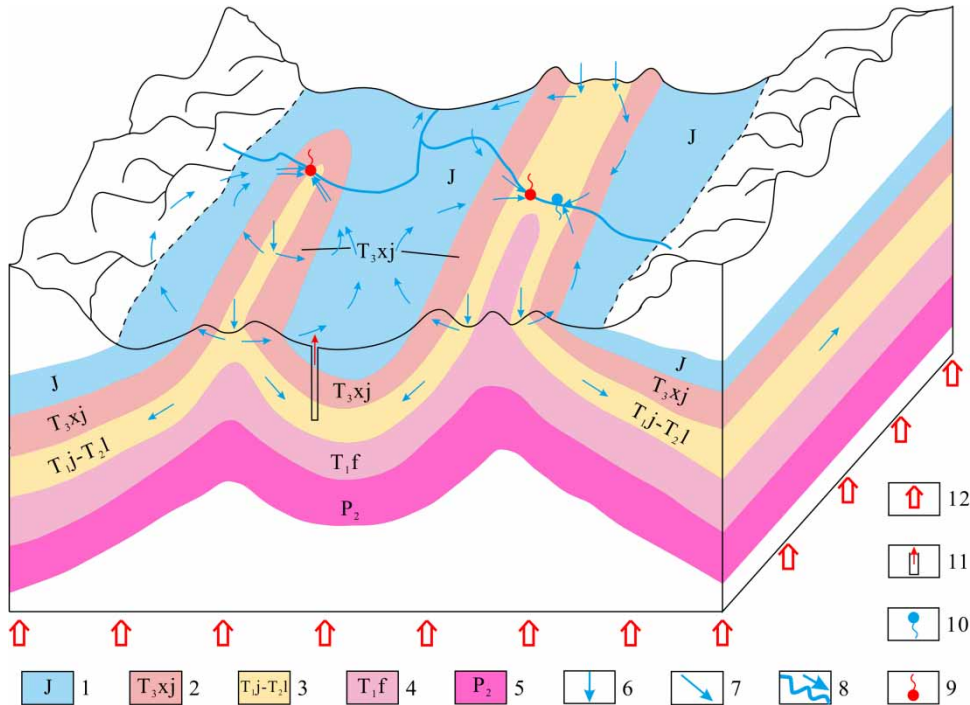
Figure 3 | Conceptual model of the geothermal water occurrence near Chongqing in eastern Sichuan Basin ('basin-anticline outcropping' type). 1 Jurassic sandstone aquiclude; 2 Sandstone aquiclude of the Upper Triassic Xujiuhe Group; 3 Carbonate aquifer of the Lower Triassic Jialingjiang and Middle Triassic Leikoupu Groups; 4 Marl aquiclude of the Lower Triassic Feixianguan Group; 5 Chert nodule limestone of the Upper Permian; 6 Infiltration of precipitation; 7 Direction of groundwater flow; 8 River; 9 Hot spring; 10 Normal temperature spring; 11 Geothermal well; 12 Heat flow.
