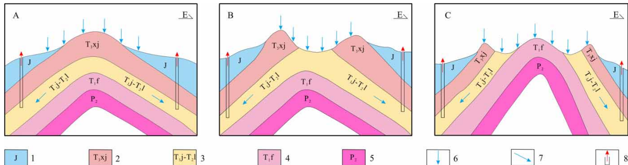
Figure 4 | Schematic cross sections showing the occurrence of geothermal water in the anticlines near Chongqing. Legends are consistent with those in Figure 3 (modified after Ta et al. (2018) and Cheng et al. (2015)).
