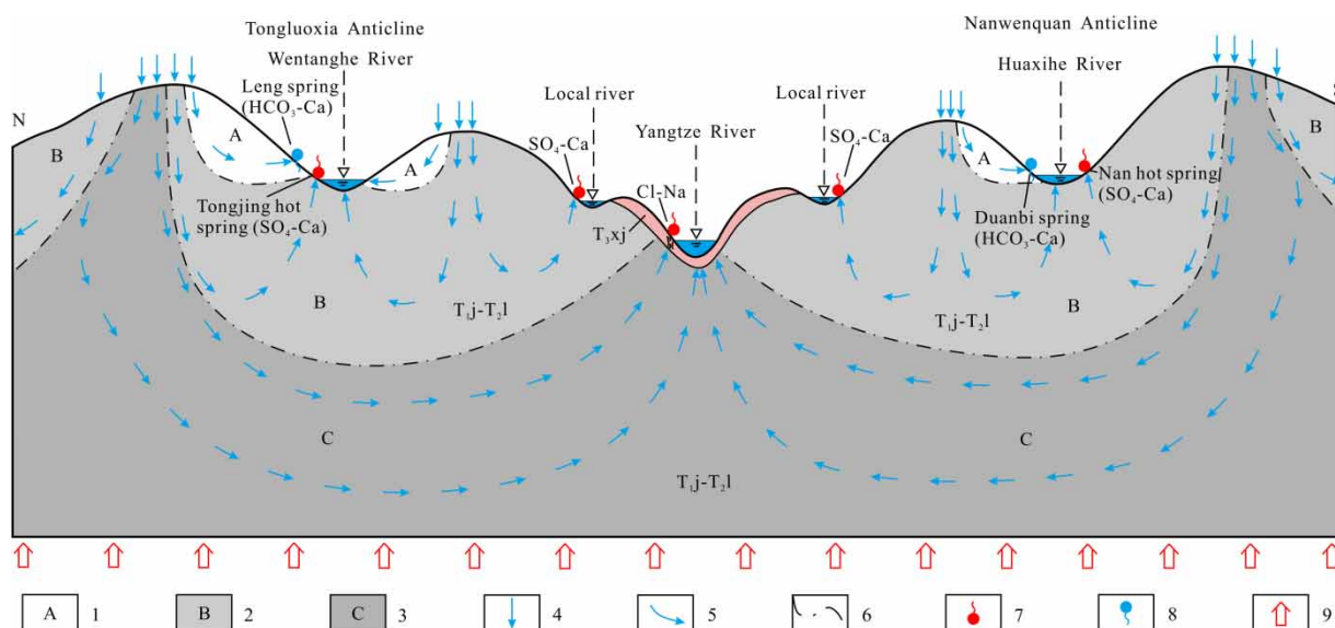
Figure 6 | Conceptual model (profile) of geothermal flow systems of the thermal groundwater along the flanks of the anticlines near Chongqing (take the Tongluoxia anticline – Nanwenquan anticline as an example). 1 Shallow circulation system; 2 Middle circulation system; 3 Deep circulation system; 4 Infiltration of precipitation; 5 Schematic groundwater flow direction; 6 Boundary of systems; 7 Hot spring; 8 Normal temperature spring; 9 Heat flow.
