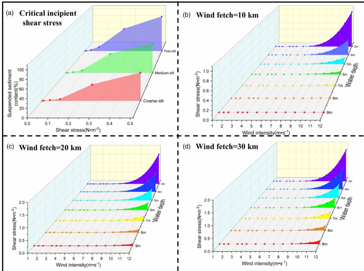
Figure 4 | (a) Relationship between shear stress and sediment suspension for fine-, medium-, and coarse-silts. (b), (c), and (d), respectively, illustrate wind's contribution to the bottom shear stress at varied water depths with the wind fetches of 10 km, 20 km, and 30 km.
