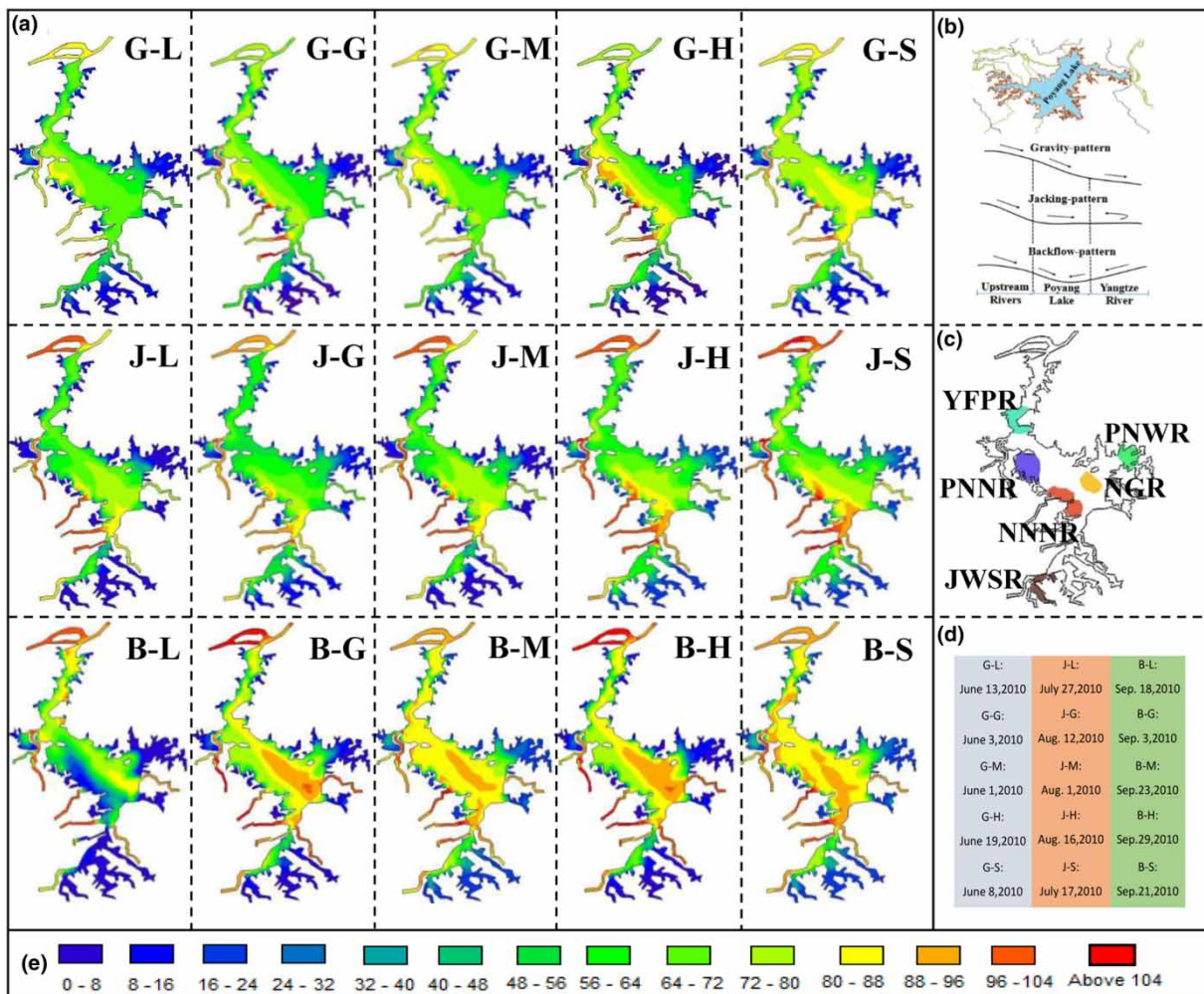
Figure 5 | (a) The SS distribution under the combination of varied currents and wind events in Poyang Lake. The two letters, respectively, indicate current pattern and wind event. (b) The flow directions under the gravity-, jacking-, and backflow-pattern current. (c) The distribution of six reserves in the computed area. (d) The dates of wind events under different current patterns. (e) The SS concentration gradient, \text{mg}/\text{L} .
