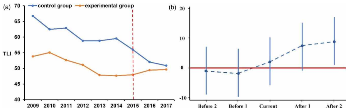
Figure 3 | Parallel trends of the eutrophication degree between the experimental group and the control group. Please refer to the online version of this paper to see this figure in color: http://dx.doi.org/10.2166/nh.2020.047 .
