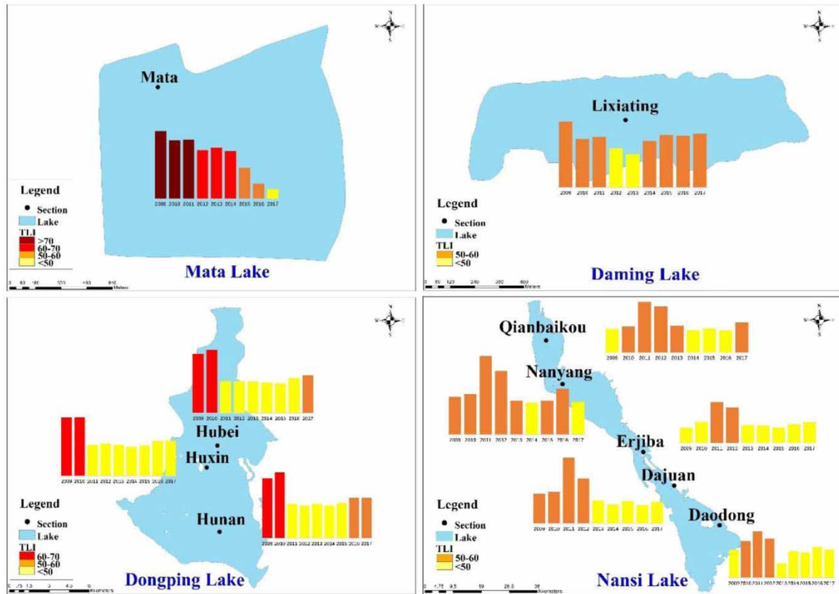
Figure 2 | Spatial and temporal variation of TLIs in 10 state-controlled sections from 2009 to 2017.
