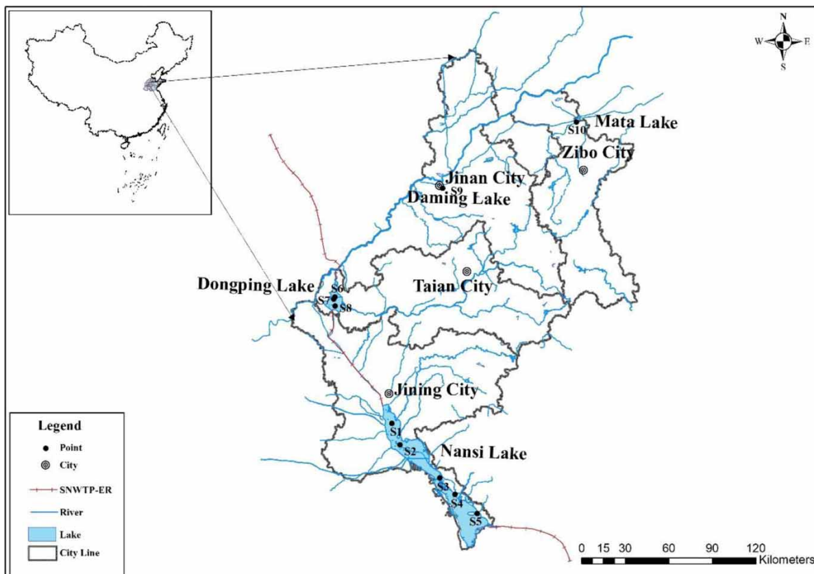
Figure 1 | Location of Nansi Lake, Dongping Lake, Mata Lake and Daming Lake and the SNWTP-ER route in the Shandong Peninsula.
