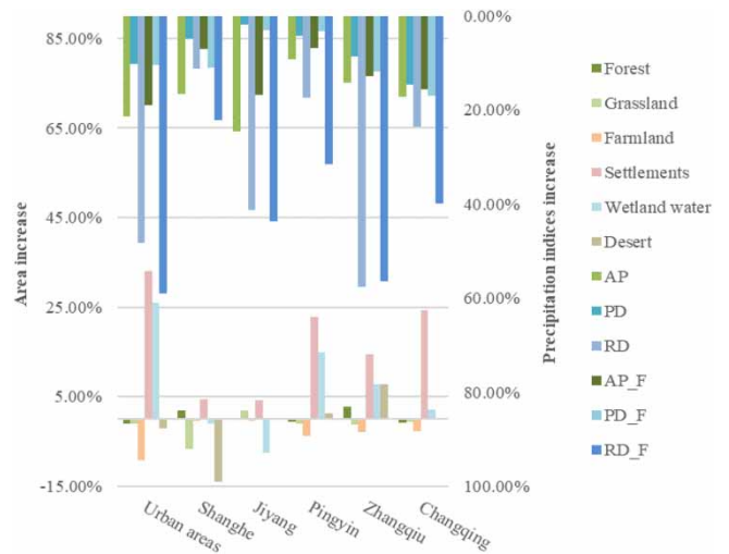
Figure 12 | The relationship between precipitation indices and land use changes in different regions of Jinan.
