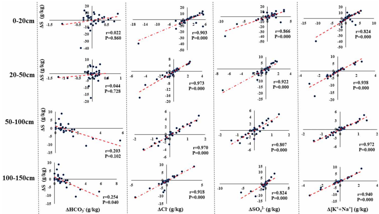
Figure 7 | The relationships between the concentration changes in main ions and soil salinity ( \Delta S ).
