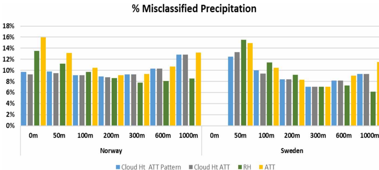
Figure 2 | Percent misclassified precipitation in Norway and Sweden for each precipitation phase parameterization method by cloud base height category.
