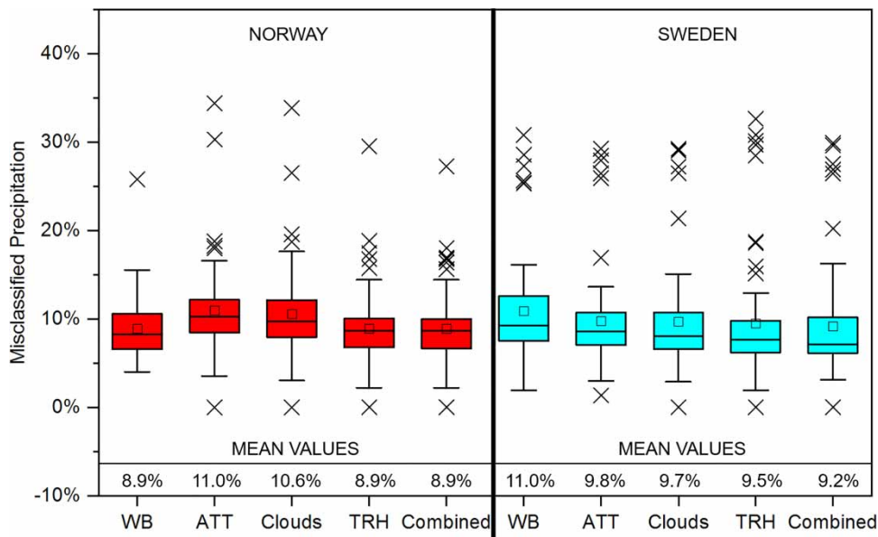
Figure 4 | Misclassified precipitation percentages for the labeled precipitation phase determination schemes in Norway (red/left) and Sweden (blue/right). Box plots cover the 25–75% probabilities with a small box indicating mean percentage, a line indicating the median value, whiskers showing the 95% confidence interval, and X marking all outliers from the 95% confidence intervals. Please refer to the online version of this paper to see this figure in color: https://doi.org/10.2166/nh.2021.072 .
