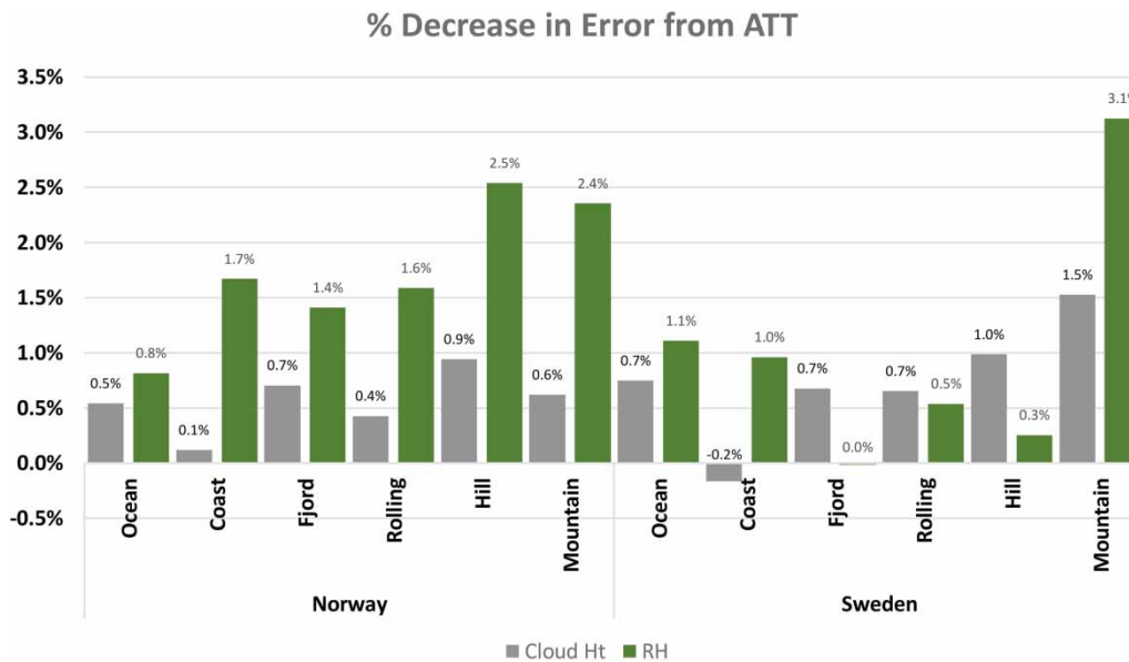
Figure 5 | Percent decrease in precipitation phase determination using T_{RH} and cloud base height ATT methods compared with a country ATTs for each identified physiographic category in Norway and Sweden.
