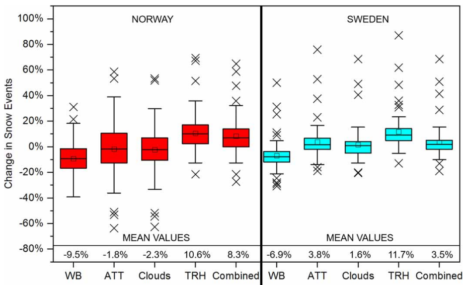
Figure 6 | Percentage change in snow events for the labeled precipitation phase determination schemes in Norway (red/left) and Sweden (blue/right). Box plots cover the 25–75% probabilities with a small box indicating mean percentage, a line indicating the median value, whiskers showing the 95% confidence interval, and X marking all outliers from the 95% confidence intervals. Please refer to the online version of this paper to see this figure in color: https://doi.org/10.2166/nh.2021.072 .
