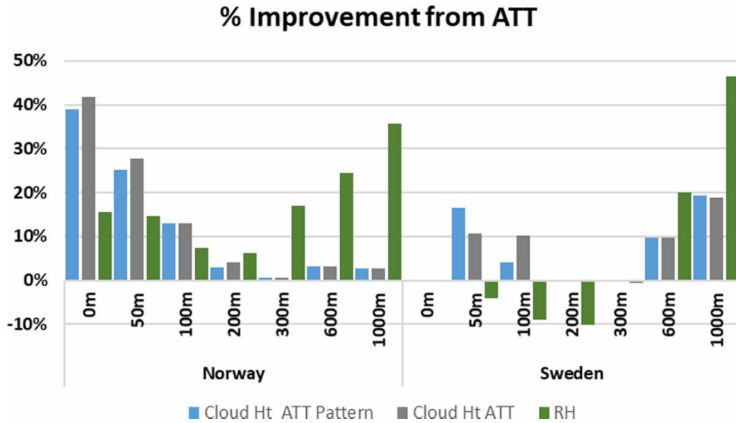
Figure 3 | Percent improvement for each cloud base height category in Norway and Sweden using cloud base height and RH precipitation phase determination methods.
