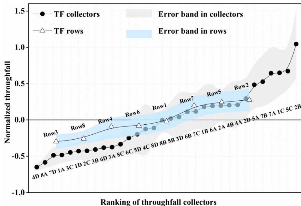
Figure 5 | Time stability plots of normalised throughfall to zero mean at unit variance and in each row are shown for total event. Thirty-two plots consist of eight rows (1–8) and four columns (A–D) of TF collectors. The number–letter names (row–column) of the TF collectors below the figure are ranked by their means in the plot. Error bands represent \pm SE.
