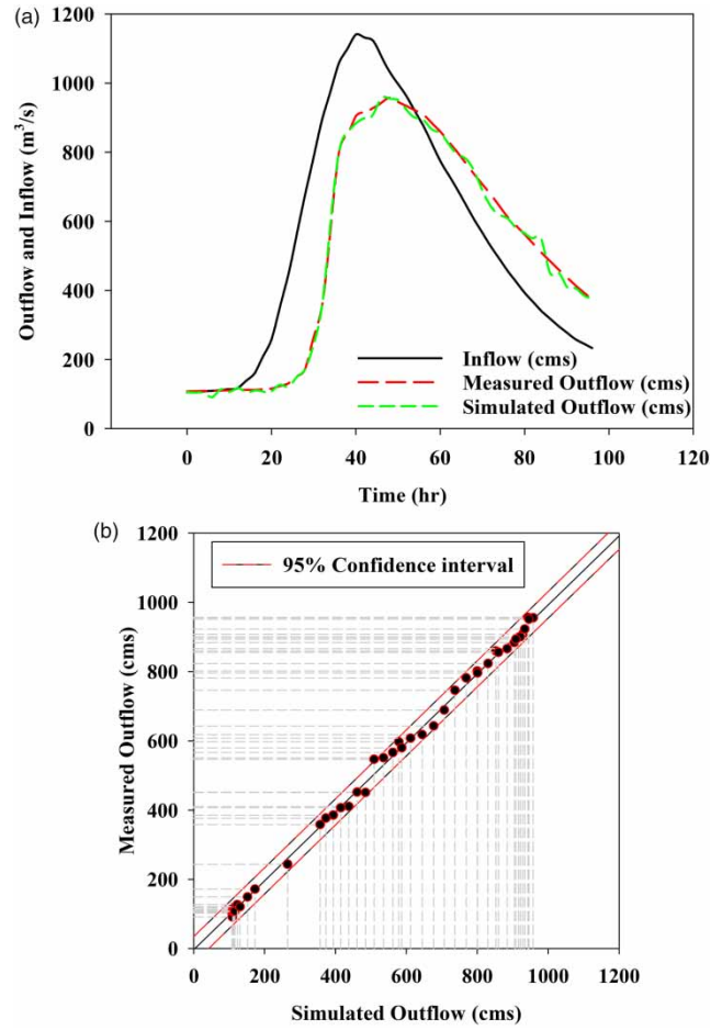
Figure 6 | Simulation results of the outflow hydrograph of the KRF (a) and 95% confidence interval of the simulation results (b) using the proposed copula-based approach.
