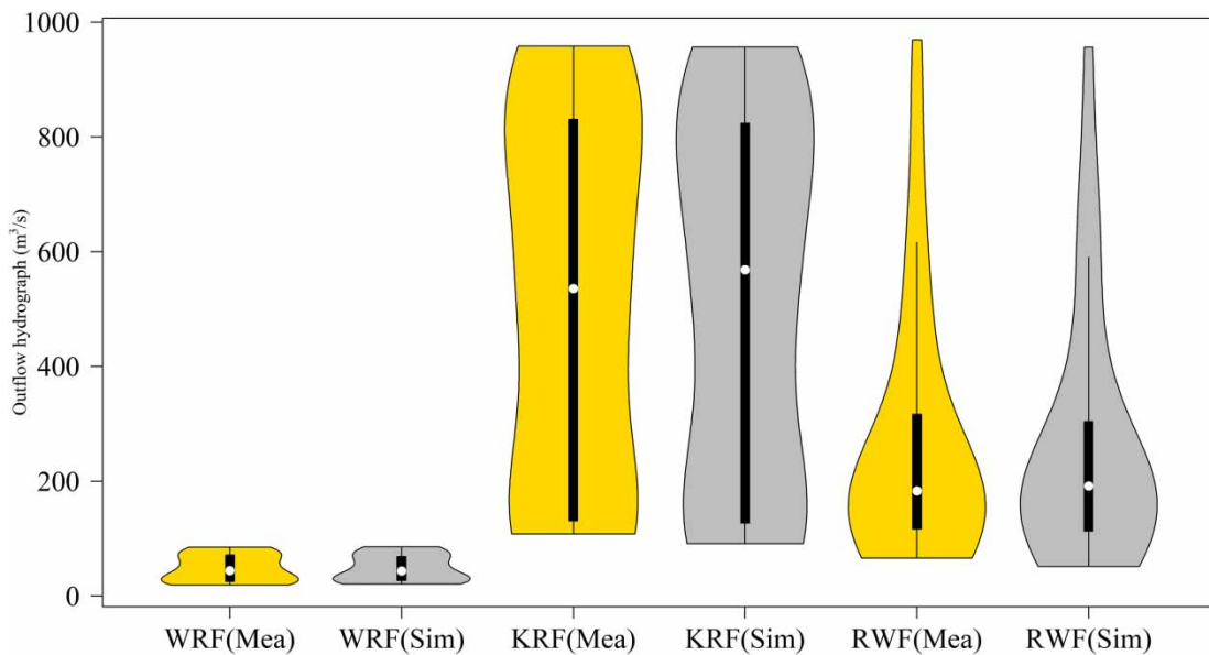
Figure 7 | Violin plots of measured (Mea) and simulated (Sim) outflow hydrographs for the case studies.
