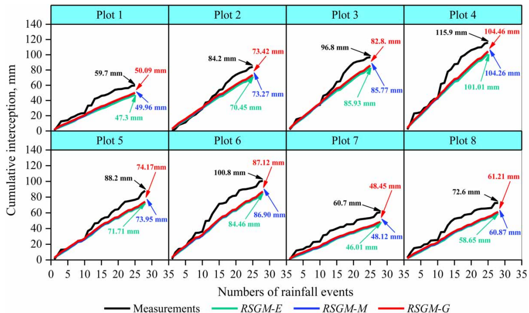
Figure 2 | Comparison among three versions of the modeled interception for each plot. The tree species in plots 1–4 are Pt , those in plots 5 and 6 are Po , and those in plots 7 and 8 are At . Arabic numerals appended to the arrowed lines represent cumulative interception values computed by different versions of the model.
