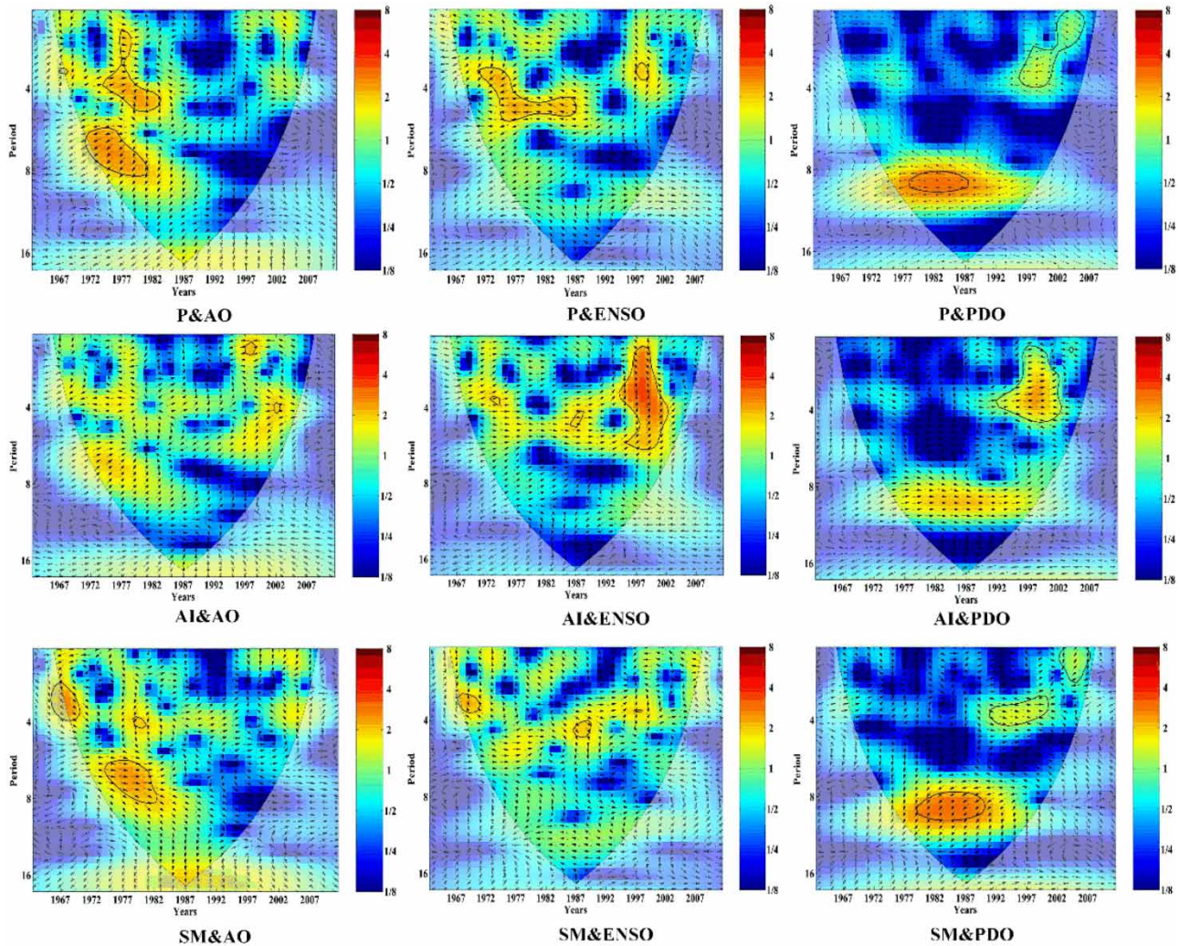
Figure 4 | Cross-wavelet of meteorological drought, underlying surface features and teleconnection factors exceeding the significance level in autumn.
