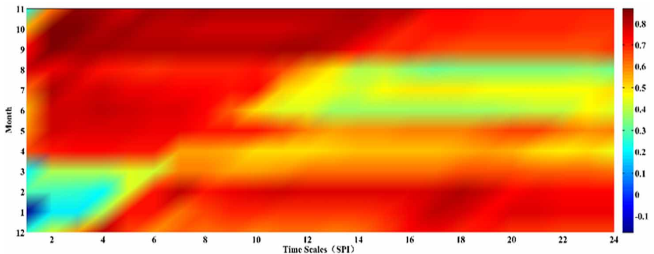
Figure 2 | Relationship between the 1-month SRI and the SPI at different time scales in the WRB. Please refer to the online version of this paper to see this figure in colour: http://dx.doi.10.2166/nh.2021.006 .
