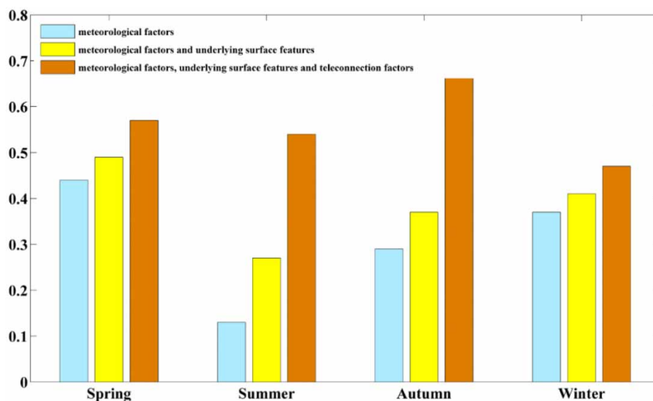
Figure 5 | Determination coefficient ( R^2 ) and significance of the multiple linear regression model between propagation time and influencing factors. '*' represents significance at the 95% confidence level.
