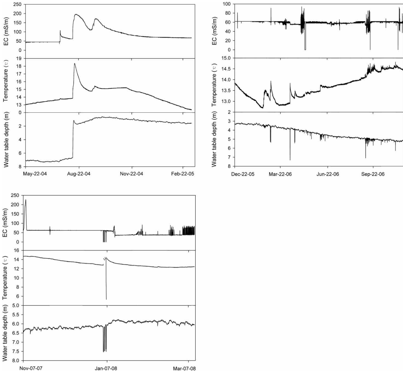
Figure 8 | Dynamic of groundwater depth, temperature and EC in well W7. Time interval is 30 minutes. A sharp rise of water level on August 12, 2004 was evidence of bed percolation. For the most part, the water level did not respond to precipitation beneath the mountain slopes even during rainy seasons (June–August). For pumping from W7, the water level declined rapidly and then stabilized at approximately 7.5 m below ground. Water level rebounded at a decreasing rate once pumping ceased.
