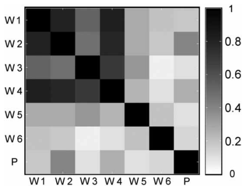
Figure 5 | Correlation matrix for time series of water table depths and precipitation. Lable P means precipitation every 10 days.
