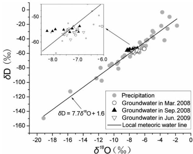
Figure 3 | Isotope composition of groundwater and precipitation.
