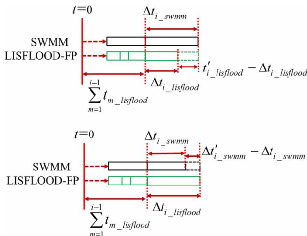
Figure 1 | Timing synchronization between SWMM and LISFLOOD-FP.
