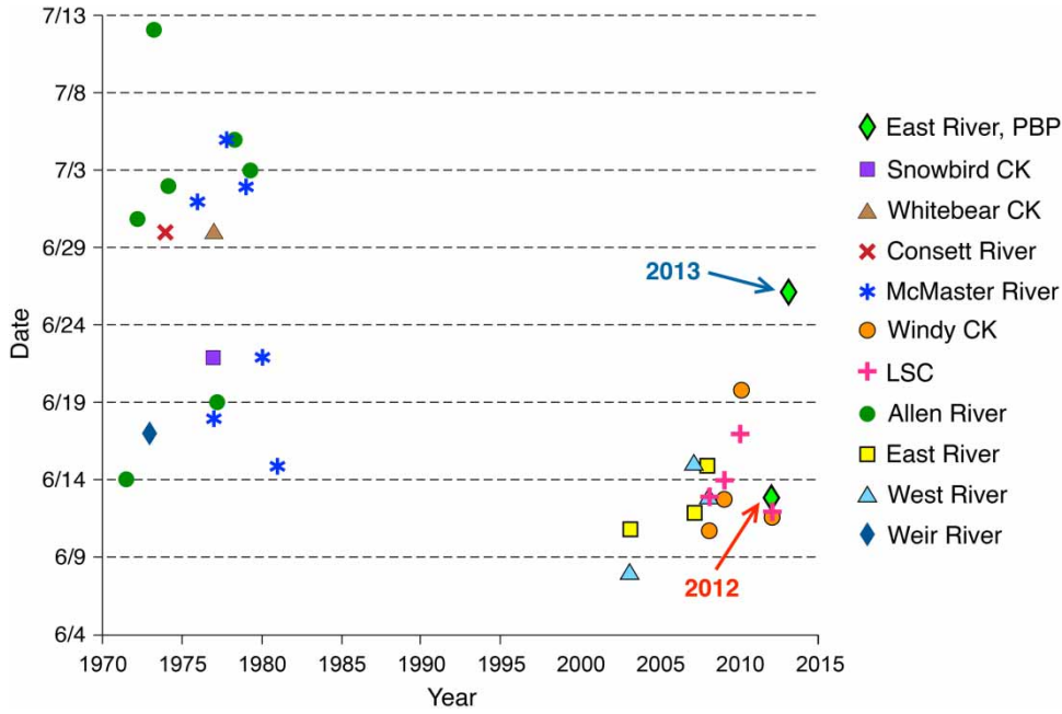
Figure 5 | First day of flow for PBP from the eastern sector watershed (East River, PBP) in comparison to other catchment and watershed studies. Diagram adapted after Young et al. (2015) . Details about watersheds other than East River, PBP can be found in Young et al. (2015) . 2003/2004 data for West and East Rivers, Cape Bounty are taken from Stewart & Lamoureux (2011) . Arrows indicate first day of flow for the East River, PBP in 2012 and 2013.
