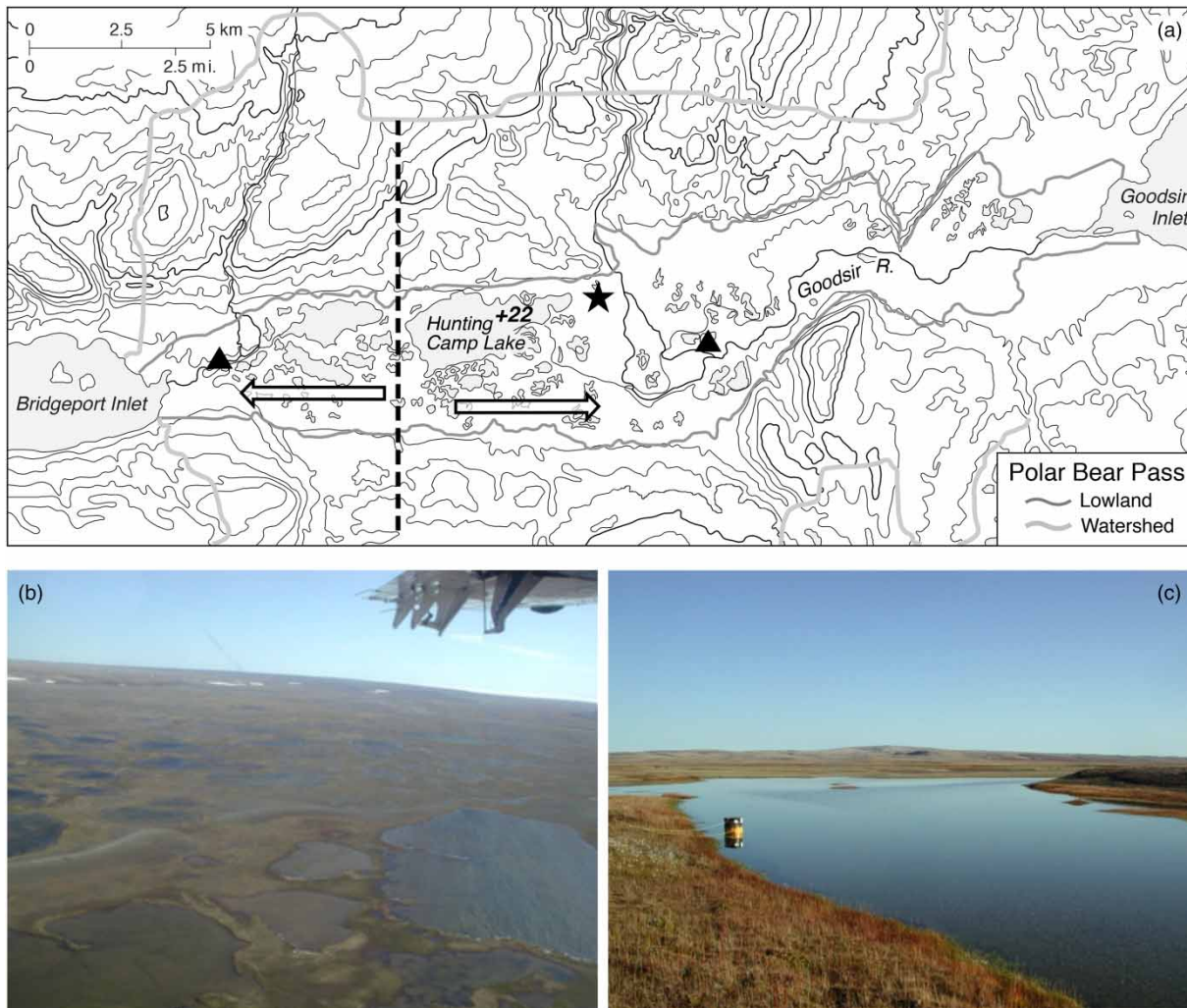
Figure 2 | Detailed map of PBP study watershed (a) including wetland and upland region. Elevation of Hunting Camp Lake is 22 m. a.s.l. and contours are 10 m (source: Young et al. 2013 ). The vertical dashed line signals the 'likely' drainage divide in the watershed. The eastern sector drainage area is estimated to be 102.6 km 2 . The star indicates the wetland Automatic Weather Station (AWS). Flow direction (arrows) and wetland outlets (triangles) are also indicated. Aerial view of the wetland (b) and photograph of the eastern outlet (gauging location) (c) taken on 4 July, 2012 are also provided.
