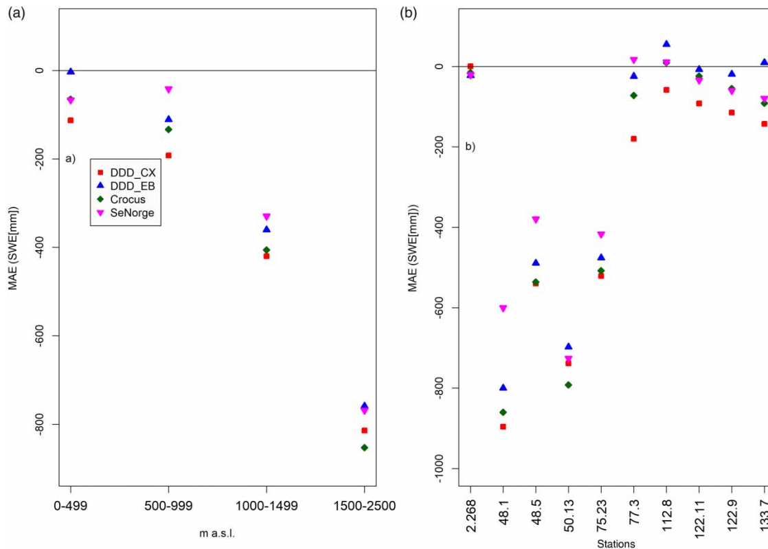
Figure 2 | Mean absolute error (MAE) of SWE simulations organised by (a) elevation and by (b) catchment.
