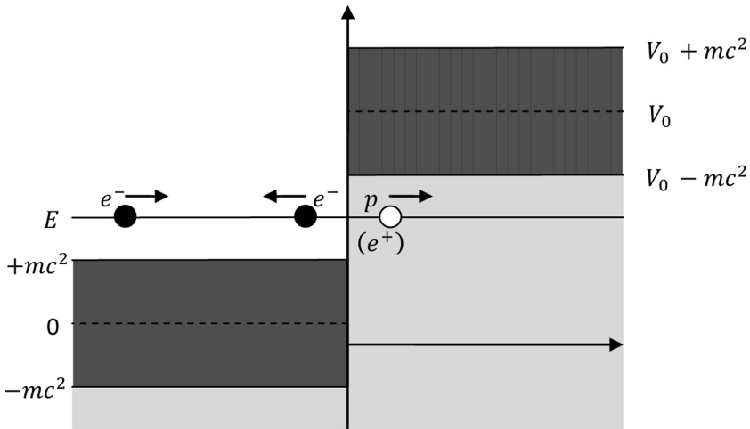
Figure 2. The Klein Paradox (Resolution). The electron current moving to the left is now accompanied by a ‘hole’ moving to the right, which is interpreted as a proton (later positron).
