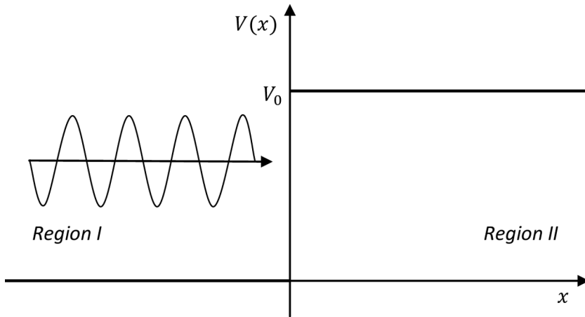
Figure 1. The Klein Paradox (Setup). An electron approaches a step potential from the left.
