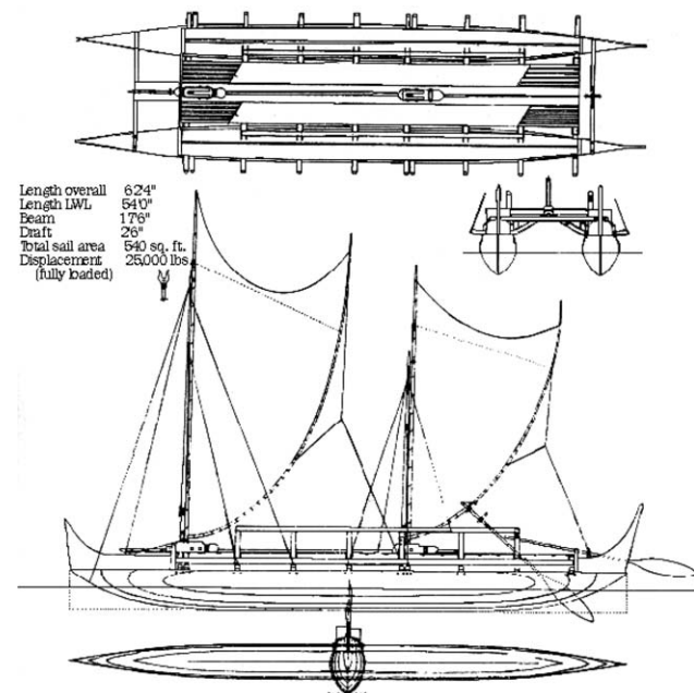
Figure 1. Original construction drawings for the Hōkūle‘a. From “Founding the Polynesian Voyaging Society; Building Hōkūle‘a,” by Ben Finney ( http://archive.hokulea.com/like/kalai_waal/finney_building_hokulea.html ). © Polynesian Voyaging Society, reprinted with permission.
